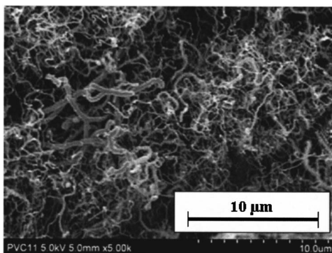
FIG. 3. SEM micrograph of CNTs grown on rolled and low temperature annealed (500 °C, 3 h), mechanically ground, constantan substrate.
