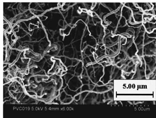
FIG. 5. SEM micrograph of CNTs grown on as-rolled, mechanically ground constantan substrate.
