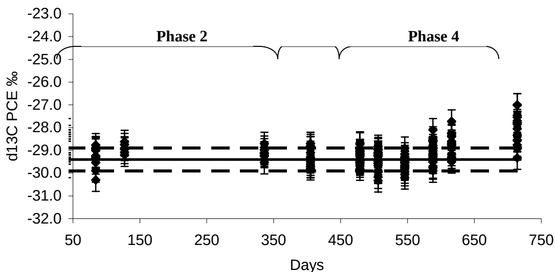
Figure 12. Isotope values of PCE during each phase of the study from all sampling locations. Error bars on d13C represent \pm 0.5\% accuracy and reproducibility of CSIA. The solid line represents the d13C of the PCE DNAPL, while dotted lines represent \pm 0.5\% error.
