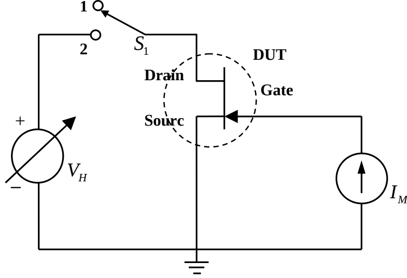
Figure 13. Thermal resistance measurement circuit.
