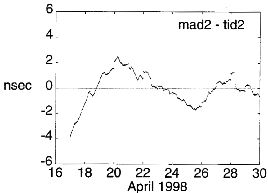
Figure 3: The Madrid, Spain clock solution minus the Tidbinbilla, Australia clock solution, for April 17-30, 1998. The difference has been de-trended (the slope is about 7 \text{ nsec/day} \approx 8 \times 10^{-14} ). Except for the 0.2-nsec-level shifts – due to 1-day processing boundaries – the solution is smooth at the 20-psec level.
