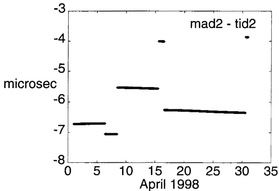
Figure 2: The Madrid, Spain clock solution minus the Tidbinbilla, Australia clock solution, during April, 1998. The difference is piecewise linear with occasional \mu\text{sec} -level shifts. The shifts are presumably symptoms of changes at one or both of the sites.
