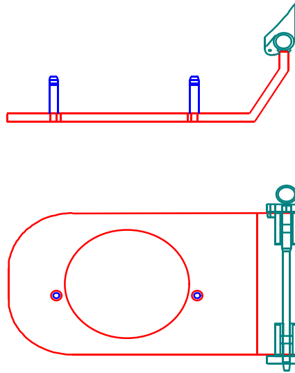
Figure 10. Spider Hinge
