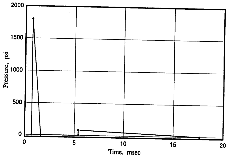
Figure 2. Design Blast Pressure History of the Cylindrical Shell
