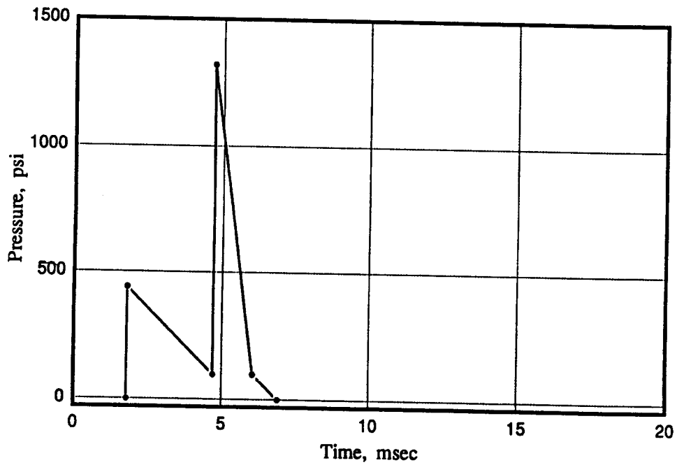
Figure 3. Design Blast Pressure History for the End Caps
