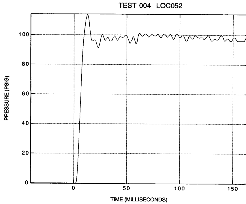
Figure 15. Quasi-Static Pressure Measured on Explosion Proof Test
