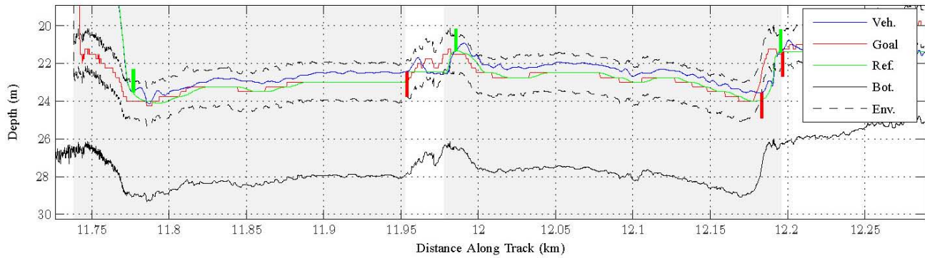
Fig. 12. Terrain-follower performance versus distance travelled during a mock photo-survey at 5 m altitude. Times when the terrain-follower was actively controlling depth are indicated by the grayed areas. The algorithm autonomously modulated speed to keep the reference trajectory within a 1 m envelope throughout the majority of the survey. This included autonomous switching into foils-fixed hover allocation from level flight allocation when the desired climb angle exceeded that attainable in level flight. Mode switch times are indicated by heavy vertical bars (green: hover→flight; red: flight→hover).
