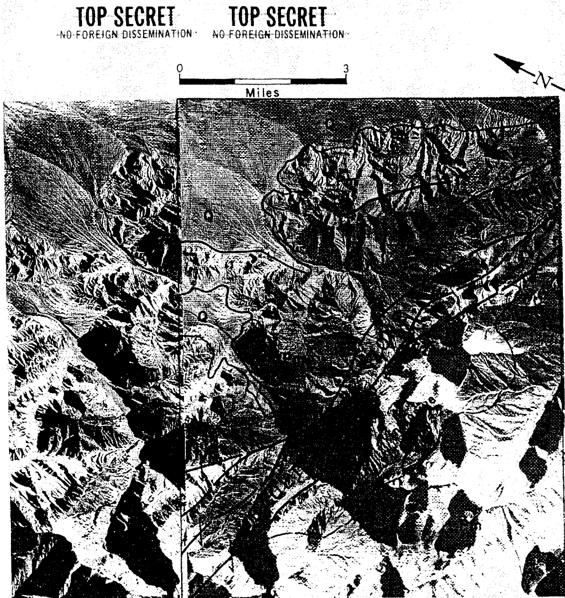
Fig. 5-5 — 3404 and SO-242 stereo pair showing apparent mineralization (red stains) in vicinity of igneous intrusion.
