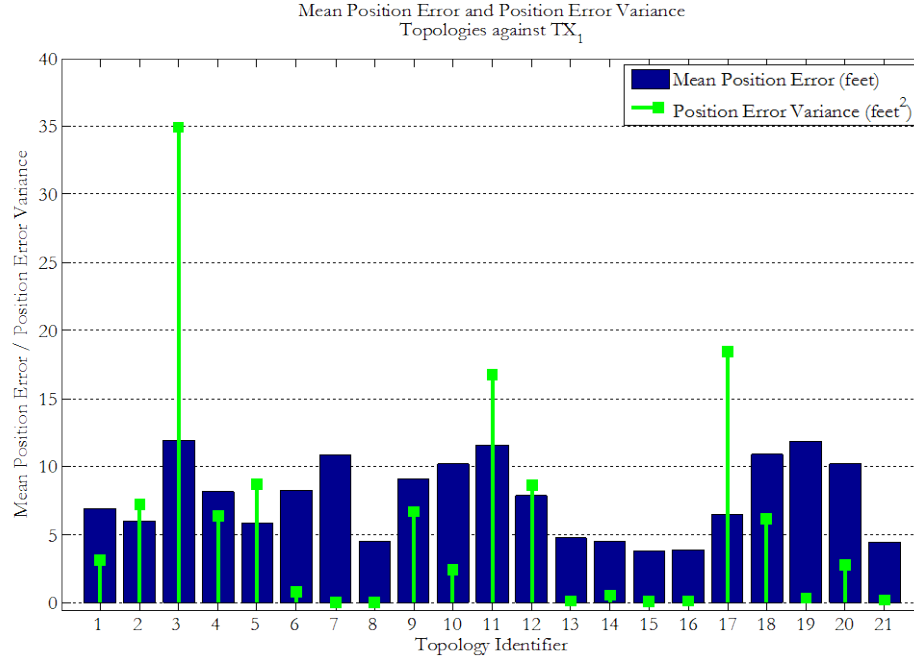
Figure 25: Mean absolute position error for all real world topologies against TX 1
