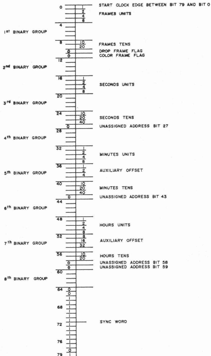
Figure 2. The 80-bit, 2400 baud Society of Motion Picture and Television Engineers (SMPTE) time code. For non-video use the time code is called "non drop-frame", and each "frame" is intended to be exactly 1/30 s. The time code uses 26 bits as binary coded decimal numerals for the frame count (0-29, the seconds (0-59 normally), the minutes (0-59), and the hours (0-23). There are six other bits reserved by the SMPTE standard, and there are 32 user bits, arranged in 8 binary groups, which can be used without restriction. The interleaving of time code and user nibbles ensures that there can be no accidentally generated 16-bit sync word for any combination of user bits. Six of the user bits have been assigned by Leith Video to code an auxiliary clock offset in binary, in half-hour increments (0-47 coding 0h to 23h 30 m).
