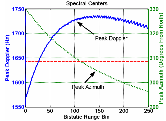
Fig. 3. Spectral centers
