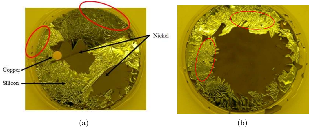
Figure 4.3: Delamination of Sprecher's nickel electroplating samples. The delamination was caused by the high tensile stress introduced during the electroplating process and began immediately after being removed from the bath. For the first sample, (a), the circles identify where the delamination began. The second sample, (b), experienced such high stress that 30 microns of substrate, identified by the circles, were ripped up with the nickel deposition [5].
