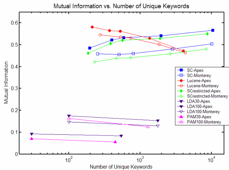
Figure 49: Summary of MI vs. Dimensionality
