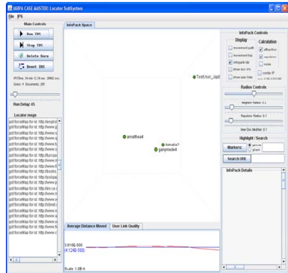
Figure 35. Display control shows only user InfoPacks.
