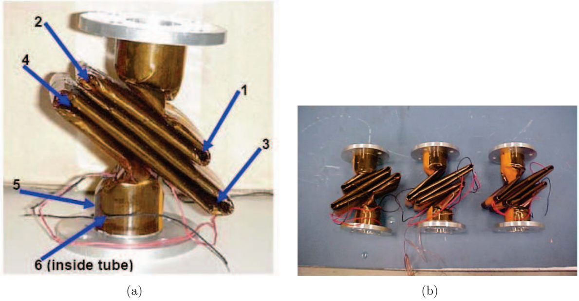
Figure 3.3: (a) Lindemuth’s tube heating profile thermocouple locations [22]. (b) Flight tubes in z-fold configuration prior to installation in RIGEX. Note the leftmost tube’s folds are 180° opposed to the other tubes. This tube is flight tube 2.
