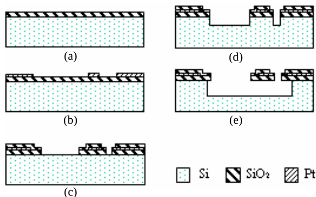
Fig.2 Fabrication process flow. (a) PECVD SiO 2 deposition. (b) Pt sputtering and lift-off to form heater and pads. (c) Top PECVD SiO 2 deposition and patterning. (d) Anisotropic Si dry etch. (e) Isotropic Si dry etch and heater release.
