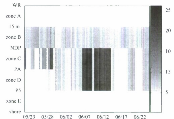
Fig. 9. Inferred time series of mud thickness in cm. This shows the solution in terms of \langle \delta_{m,0,x,t} \rangle , with \langle \rho_m, v_m \rangle held constant.
