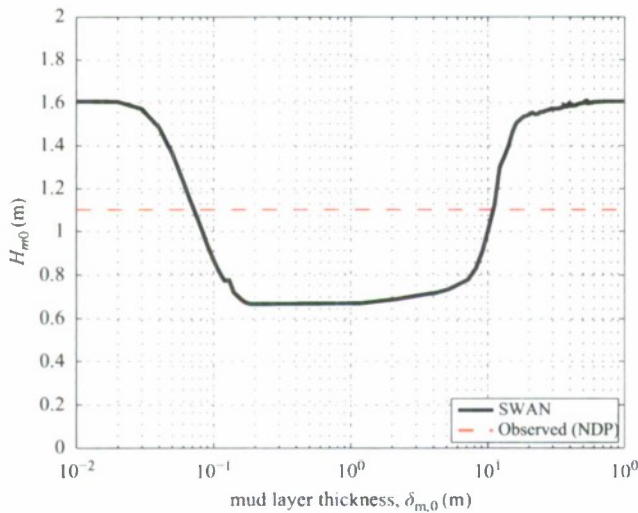
Fig. 8. Example of inferring mud thickness from wave height observation. Here, solutions of \delta_{m,0} = 0.07 and 11 m are obtained. In this case, the maximum dissipation occurs with \delta_{m,0,max} = 18.4 cm.
