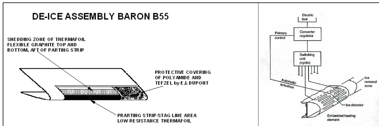
Figure 34. Graphite conductor electrothermal system by Northcoast technologies.
