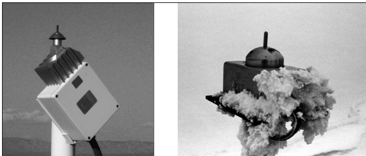
Figure 55. Rosemount ice detectors for measuring freezing rain (left) or rime ice (right).
