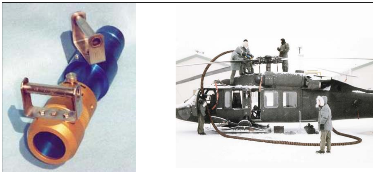
Figure 36. Buddy Start deicing nozzle (left) and system in use on Black Hawk helicopter (right).
