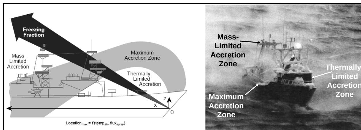
Figure 16. Zones of spray, thermal, and ice accretion processes on ships.
