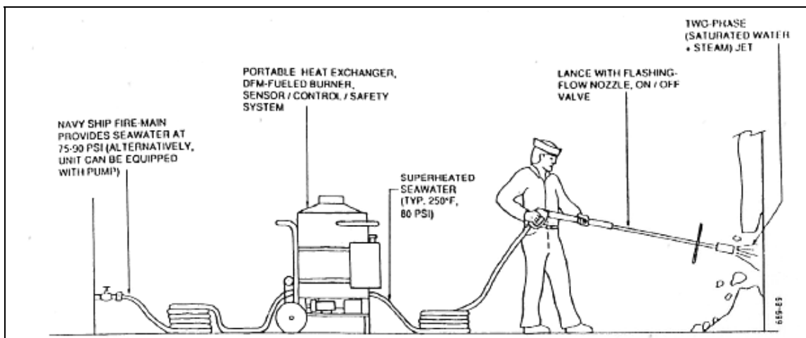
Figure 38. Flash flow portable deicing system for ships.
