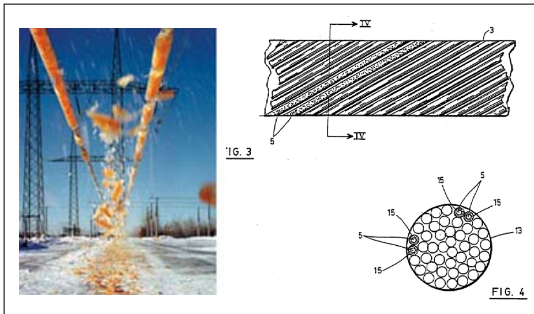
Figure 54. Electro-expulsive deicing technology applied to cables. Image on left shows colored ice falling from cables immediately after system activation.
