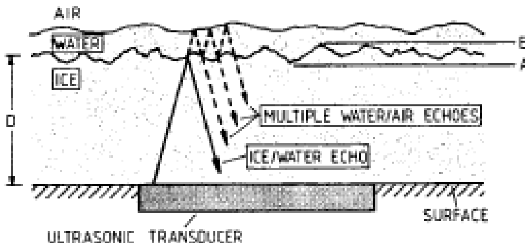
Figure 60. Operation of ultrasonic ice detectors.
