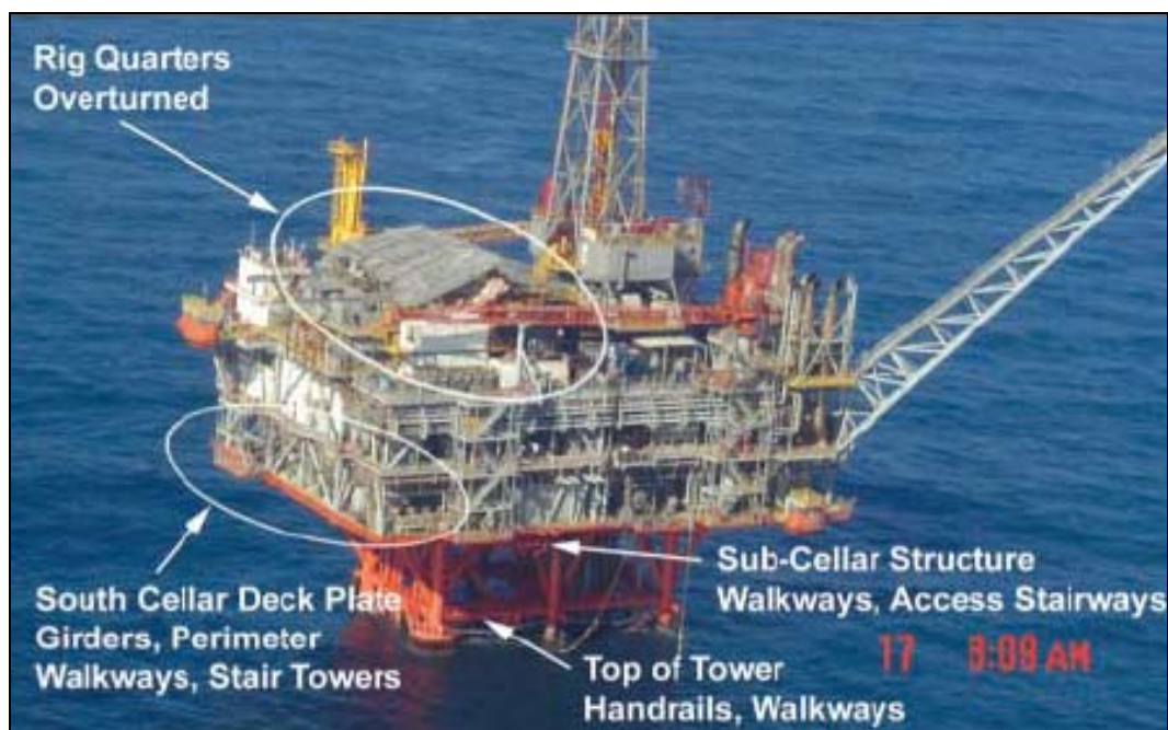
Figure 9. Complex cellar deck on the rig Petronius that would ice readily if located in colder waters.
