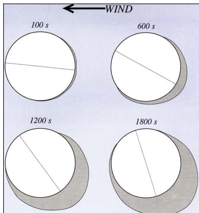
Figure 52. Rotation of cables during wind-driven icing conditions, caused by asymmetric load, allows ice to eventually envelop the entire cable circumference.
