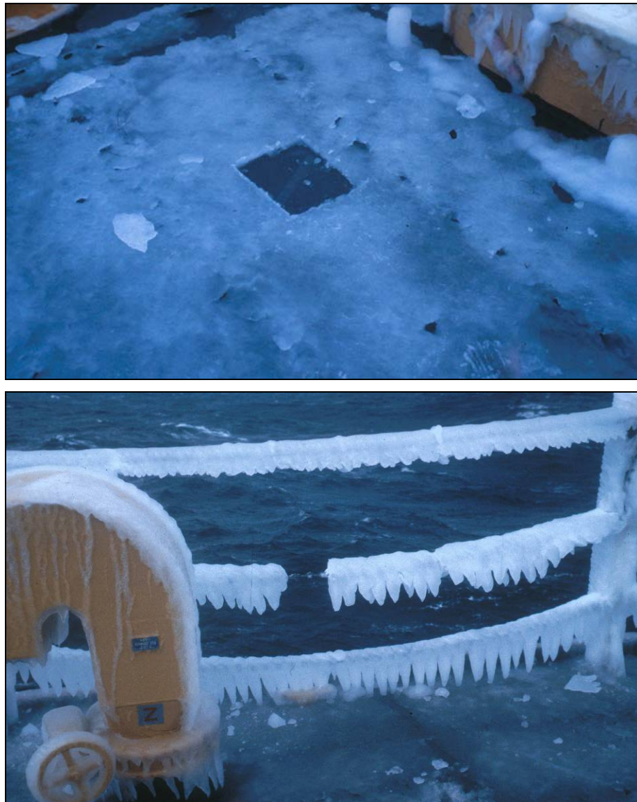
Figure 4. Superstructure ice on the Coast Guard Cutter Midgett in the Bering Sea in 1990, on the deck (top, sample removed), and on rails (bottom, sample removed).
