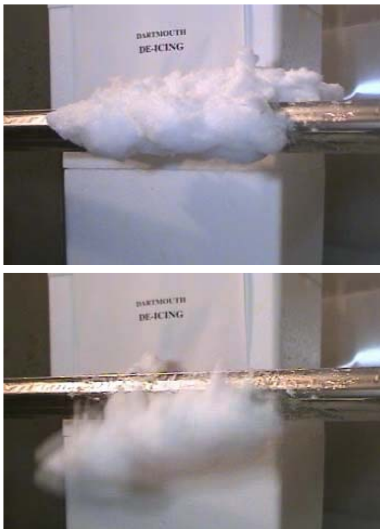
Figure 27. Ice being released from simulated cable by ice dielectric heating method.
