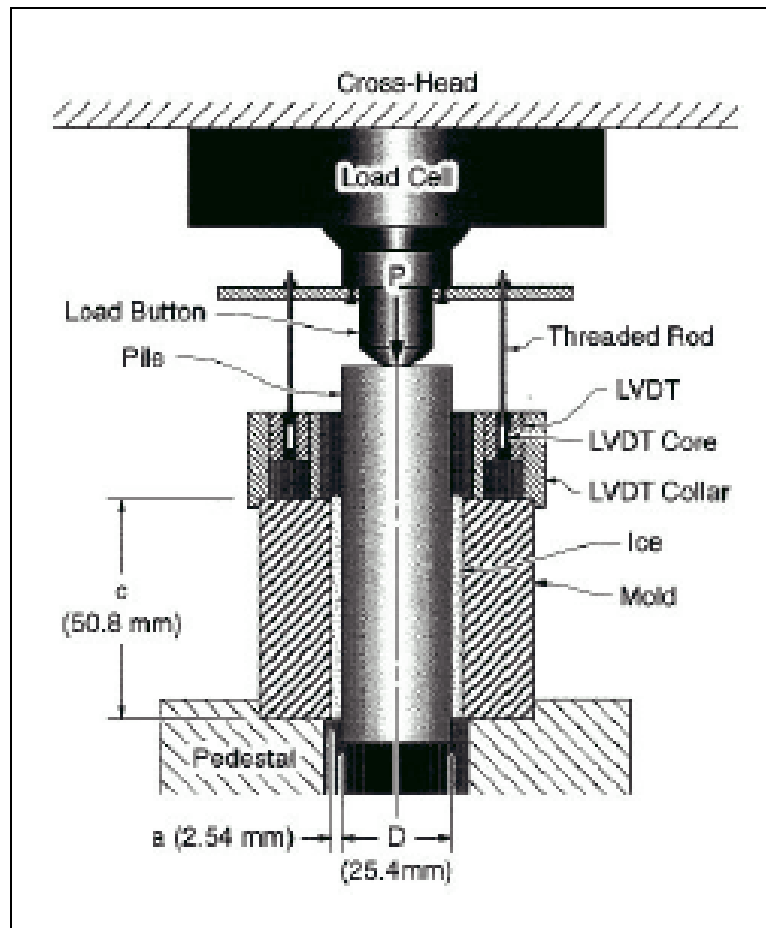
Figure 21. Mulherin and Haehnel (2003) Zero Degree Cone Test apparatus.
