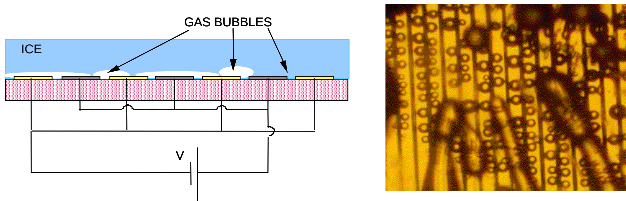
Figure 25. DC bias voltage deicing where electrolysis forms bubbles at the ice/substrate interface as seen diagrammatically in profile (left) and photographically from above (right).
