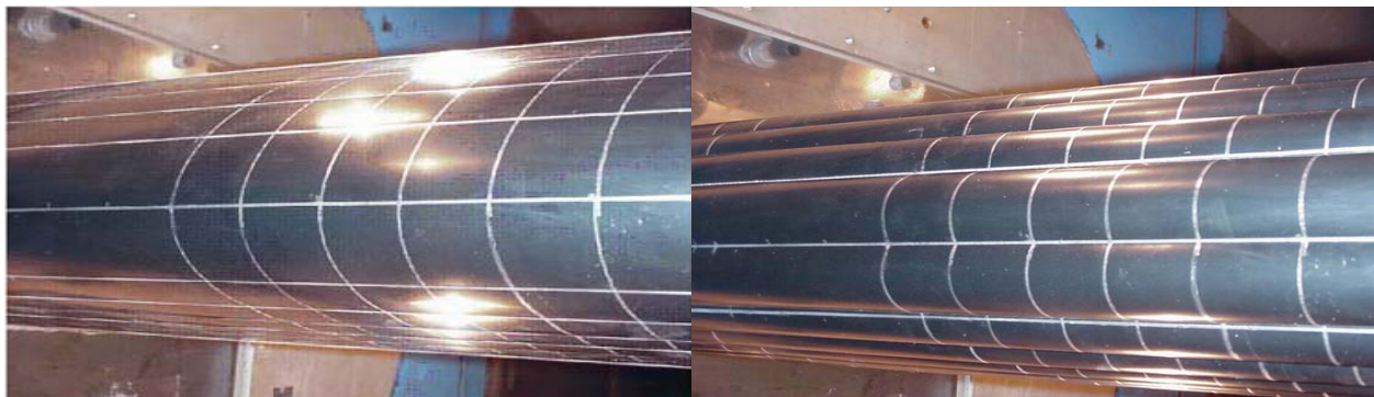
Figure 46. Diagrammatic view (top) of deflated (above) and inflated (below) deicing boot. Bottom: deflated (left) and inflated (right) boots on wing leading edge in wind tunnel.
