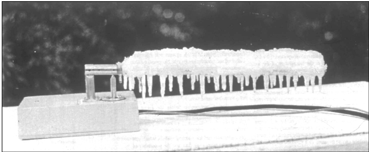
Figure 57. Pole-ice instrument for representing ice loads on transmission lines.
