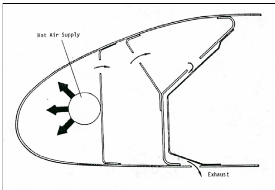
Figure 35. Piccolo tube directing hot bleed air against inside of wing leading edge.
