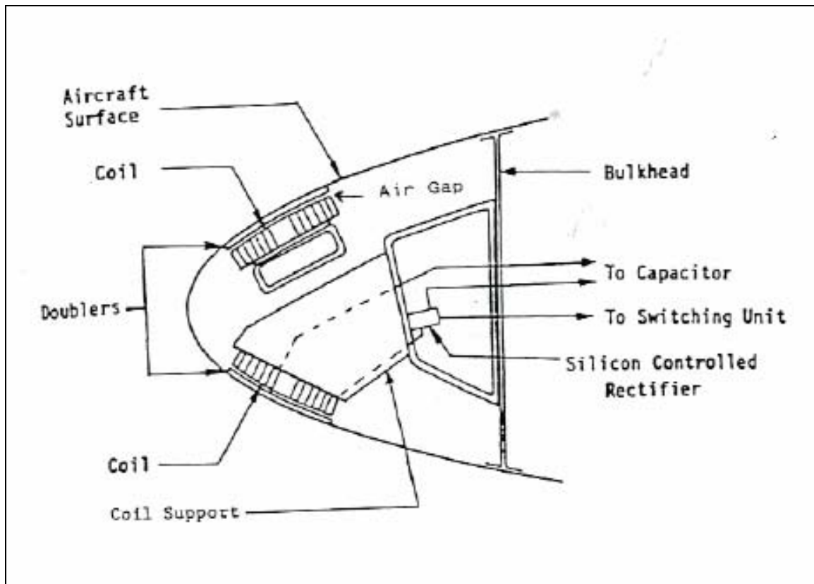
Figure 29. IDI EIDI applied to an airfoil.
