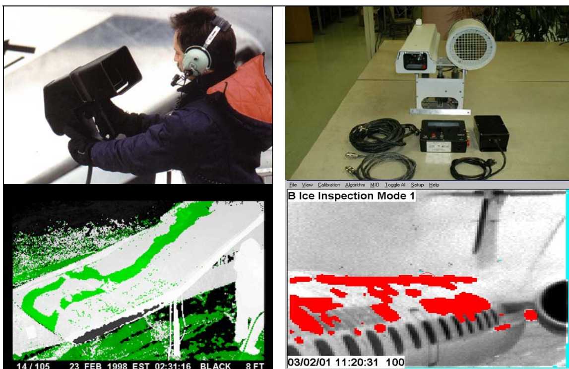
Figure 56. Ice Hawk (left images) as originally designed by RVSI, and Canadian infrared detection system (right images).
