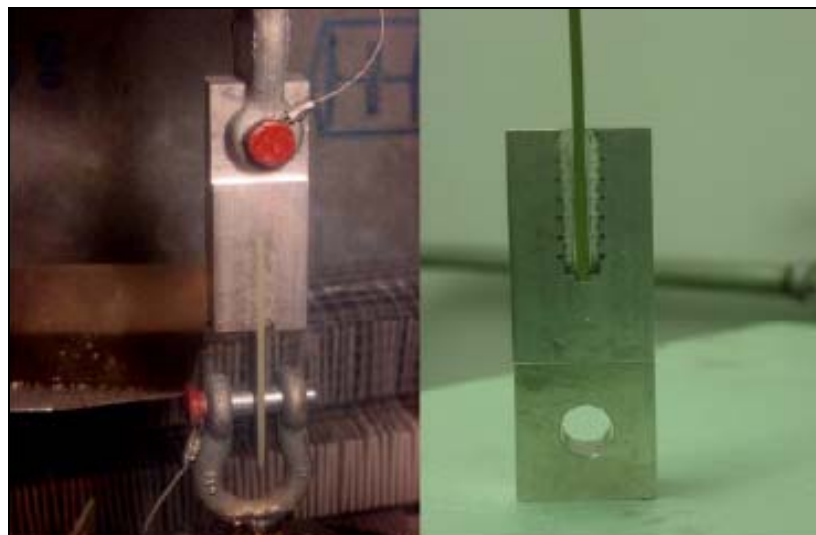
Figure 22. Ice pulled from a coupon (Ferrick et al. 2008).
