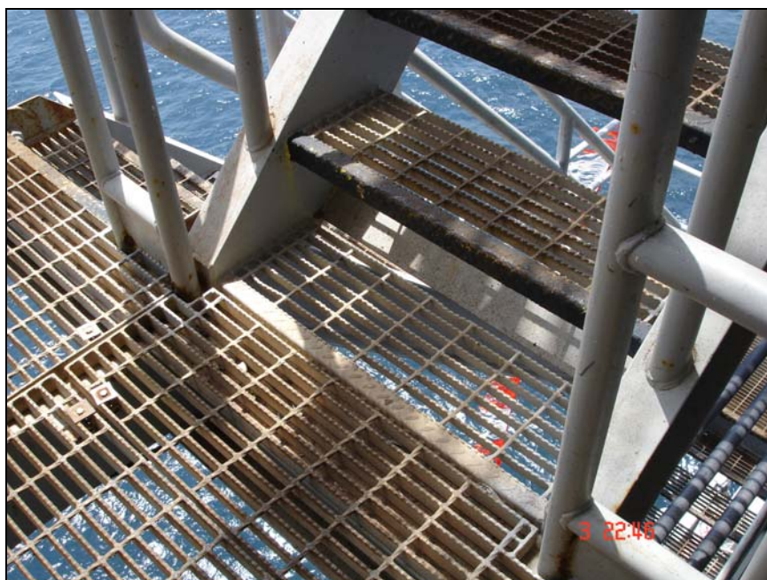
Figure 8. Open mesh walkways will accumulate ice and fill because of high collection efficiency.
