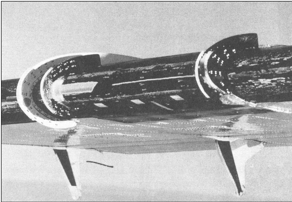
Figure 47. Residual ice occasionally remains on boots after deicing as illustrated on the boots of this NASA Twin Otter aircraft.
