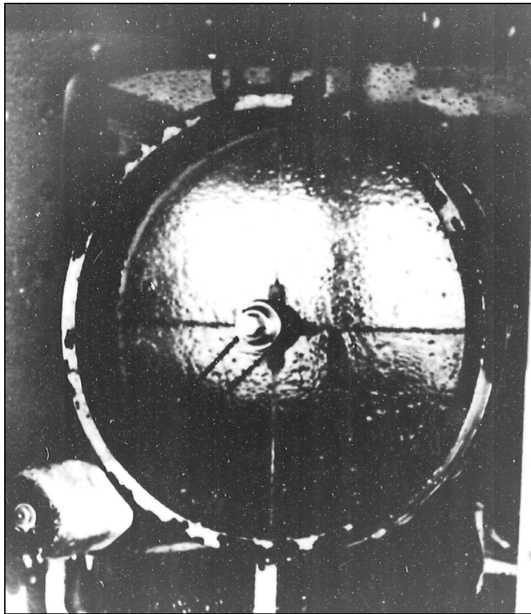
Figure 50. Ice spinning bridge window on the tug Keokuk . Spinning failed to keep the window clear.
