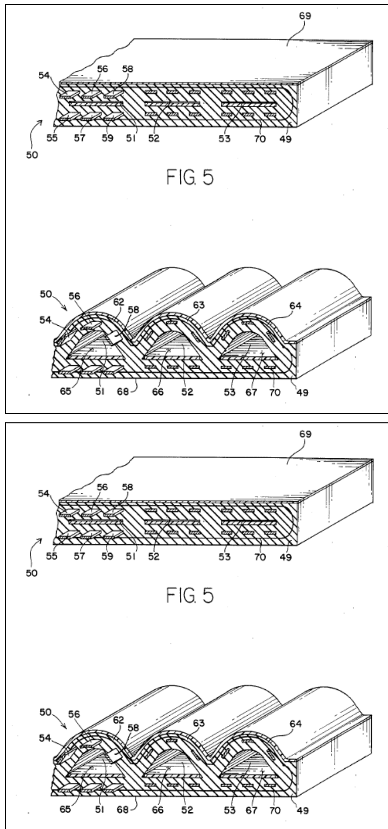
Figure 28. EEDS cross section un-actuated (above) and actuated (below).
