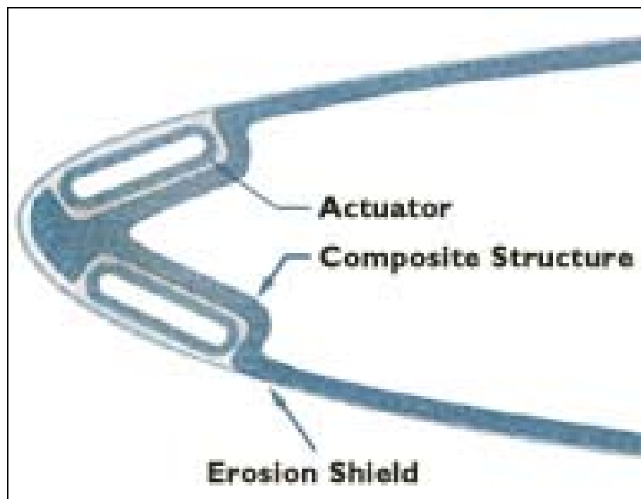
Figure 30. Cox and Company EMEDS applied to an airfoil leading edge.
