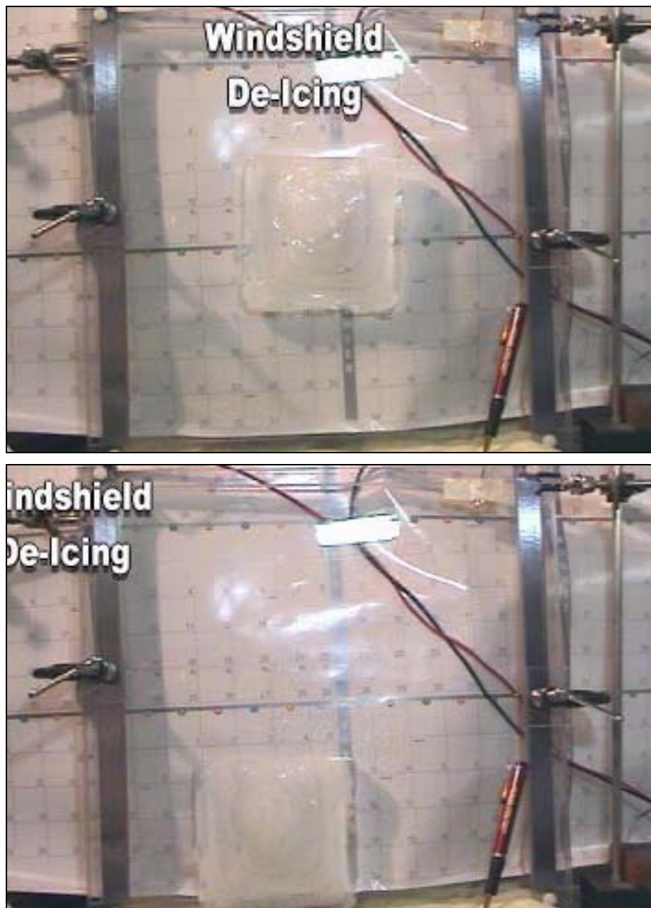
Figure 51. Pulse deicing as applied to windows. The ice sheet in the top image slid from the window after the clear conductor on the glass surface was heated rapidly.
