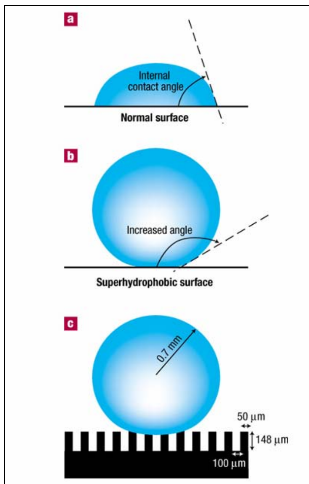
Figure 23. Drop contact angles on substrates, with lotus leaf effect at 23c.
