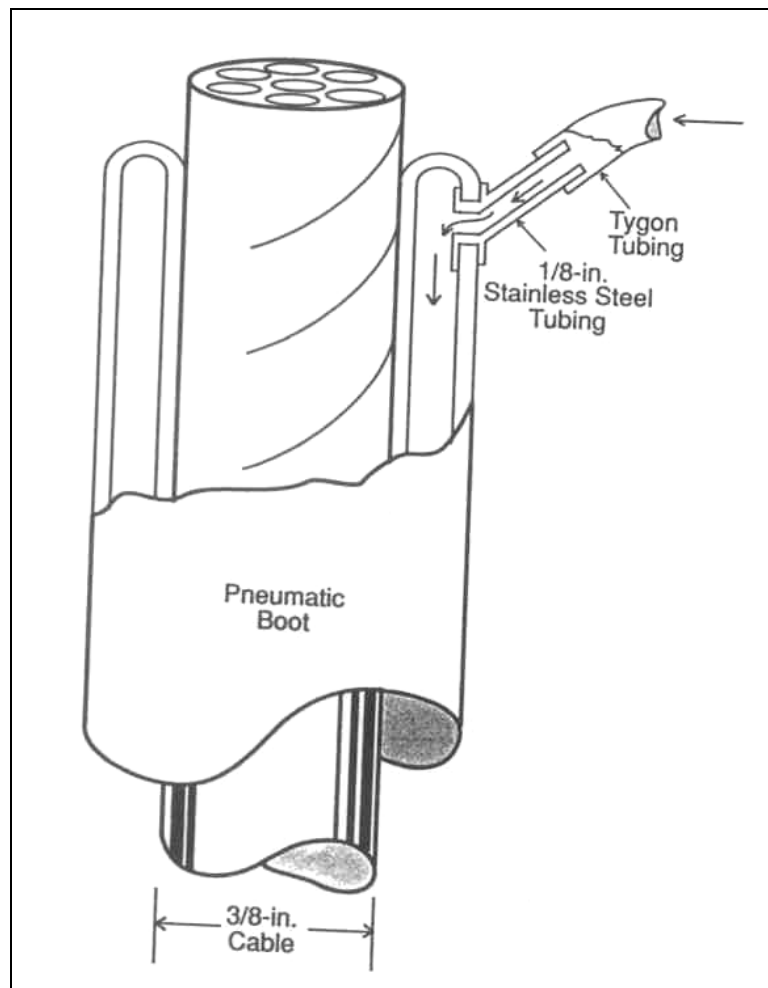
Figure 53. Pneumatic deicing boot developed by Franklin (Govoni and Franklin 1992).
