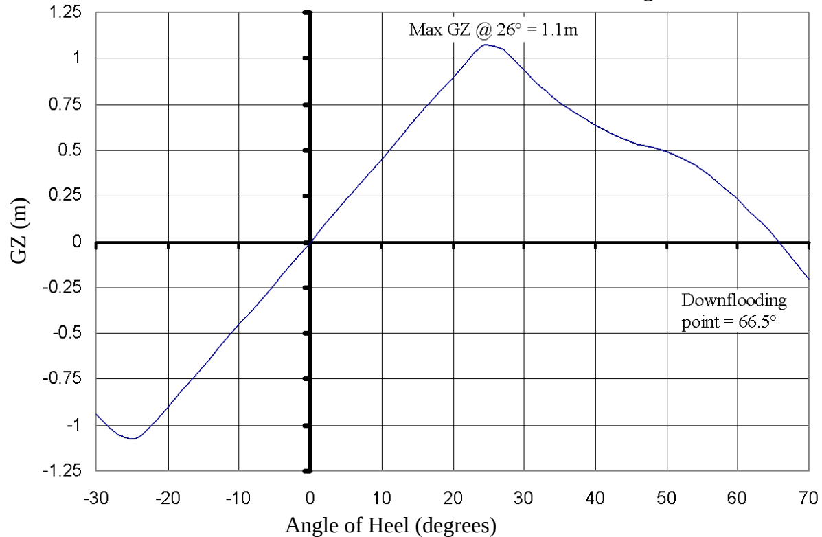
Figure 8 - GZ Curve for LSD (EFV) in Deep Condition
