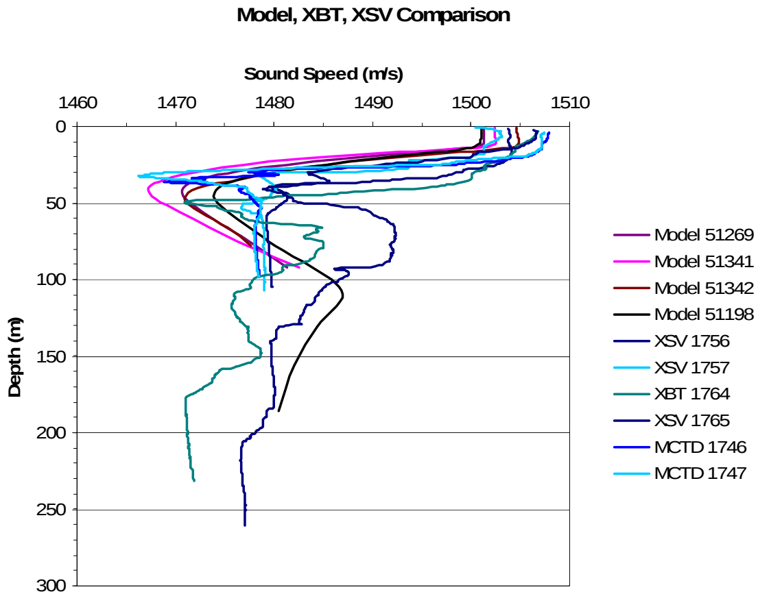
Figure 13: Sound speed comparison from four different sources. Mercator model temperature profiles from a forecast for September 17 th were used to compute the model sound speed profiles at four model locations. The in situ temperature data from the XBT and MCTD profiles were also used to compute sound speed. Finally, the XSV profiles of sound speed are included. The legend indicates the model grid location identifiers as assigned by the READB while in situ data is identified by a similar unique READB identifier.
