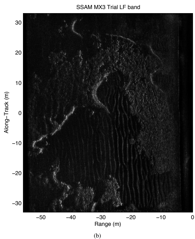
Fig. 7. Mixed posidonia, sand and mud from the Ligurian Sea
