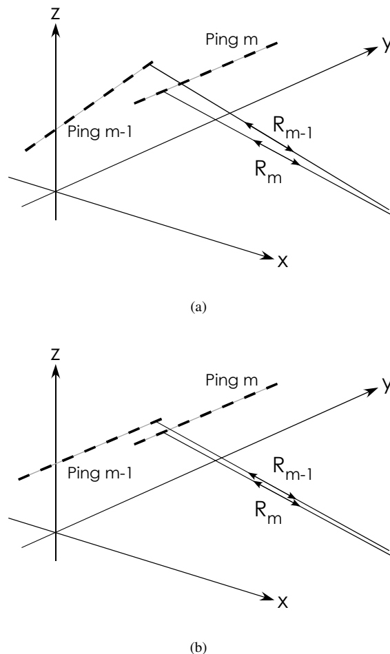
Fig. 1. The motion estimation and compensation routine used for SSAM combines angular estimates from the vehicle IMU and sway estimates from redundant phase centers. In 1(a), the array is both yawed and swayed. Using the IMU estimates we correct the array to 1(b) and then apply a sway correction based on redundant phase center delays.
