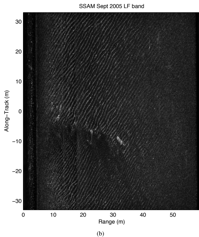
Fig. 3. Rippled sand and layered mud and sand from the Panama City, Florida Whiskey field
