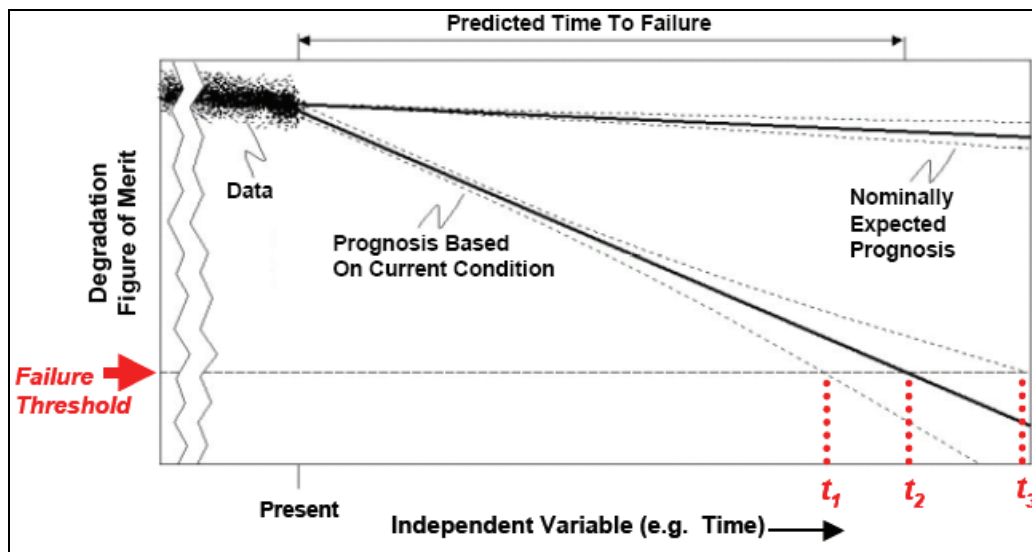
Figure 2.25. Illustration of prognostics prediction: illustrates prediction outcome of the regression models that are applied to the data sets to generate the FOMs. In this figure, a failure occurred at time t_2 with a window of uncertainty as shown by the times between t_1 and t_3 . This illustration is used to show that an accurate prediction of life usage can be obtained through the use of sensors to monitor the currently operating conditions versus estimated life usage.
