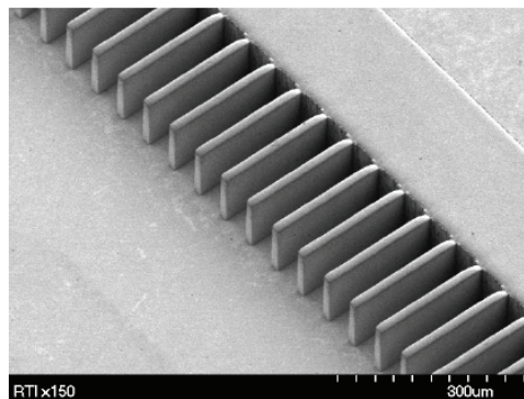
Figure 3.26. Micromachined slow wave structure for producing sub-mm wave oscillator.
