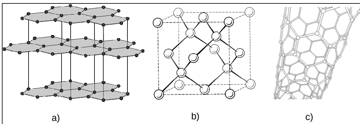
Figure 2.5. Structures of carbon as a) graphite, b) diamond, and c) nanotube.
