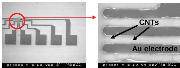
Figure 2.6. Carbon nanotube based field effect transistors (CNT diameters \sim 2 nm).
