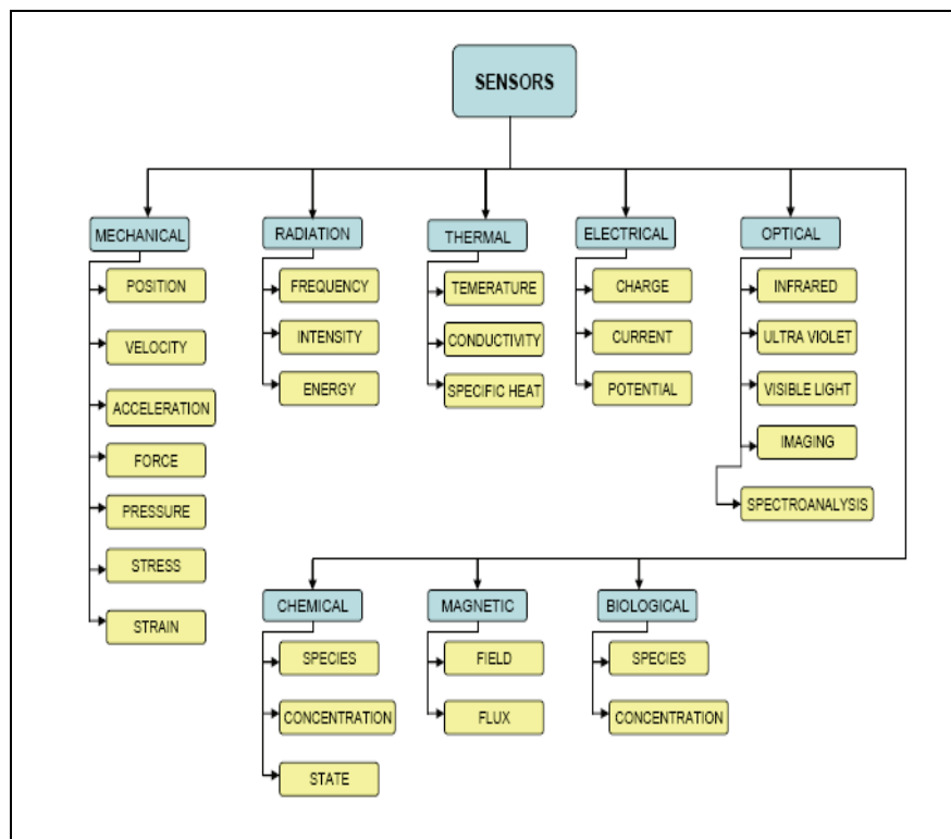
Figure 2.4. Sensor types. 19
