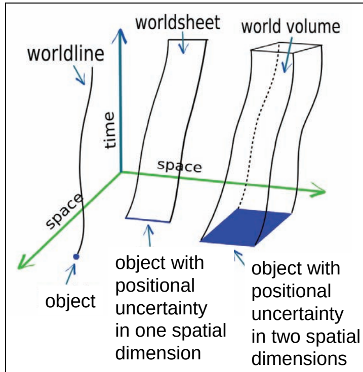
Figure 4.34. Worldline, worldsheet, and world volume as they are derived from the time-evolved states of objects with different degrees of positional uncertainty.
