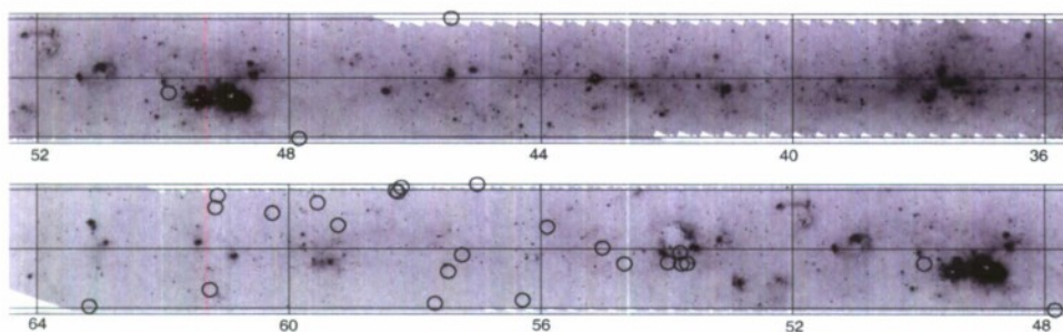
Figure 1. Location of the twenty-five newly discovered galaxies, superposed on the 24\ \mu\text{m} MIPS GAL image ( 5'' per pixel) of the Galactic plane. The top panel covers l \sim 36^\circ – 52^\circ and the bottom one l \sim 48^\circ – 64^\circ , with |b| \lesssim 1^\circ .
