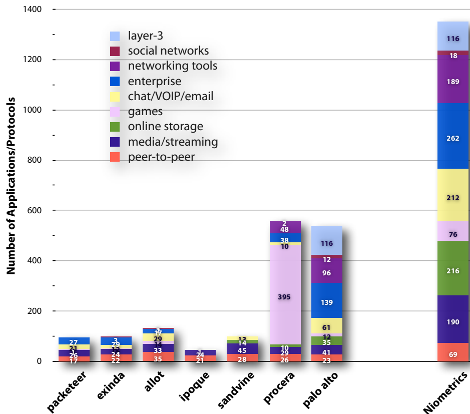
Figure 5: Comparison of application coverage between different vendors, including our own project. The resulting coverage is due to the use of our tools on reference traces and a small number of live networks and trial sites.
