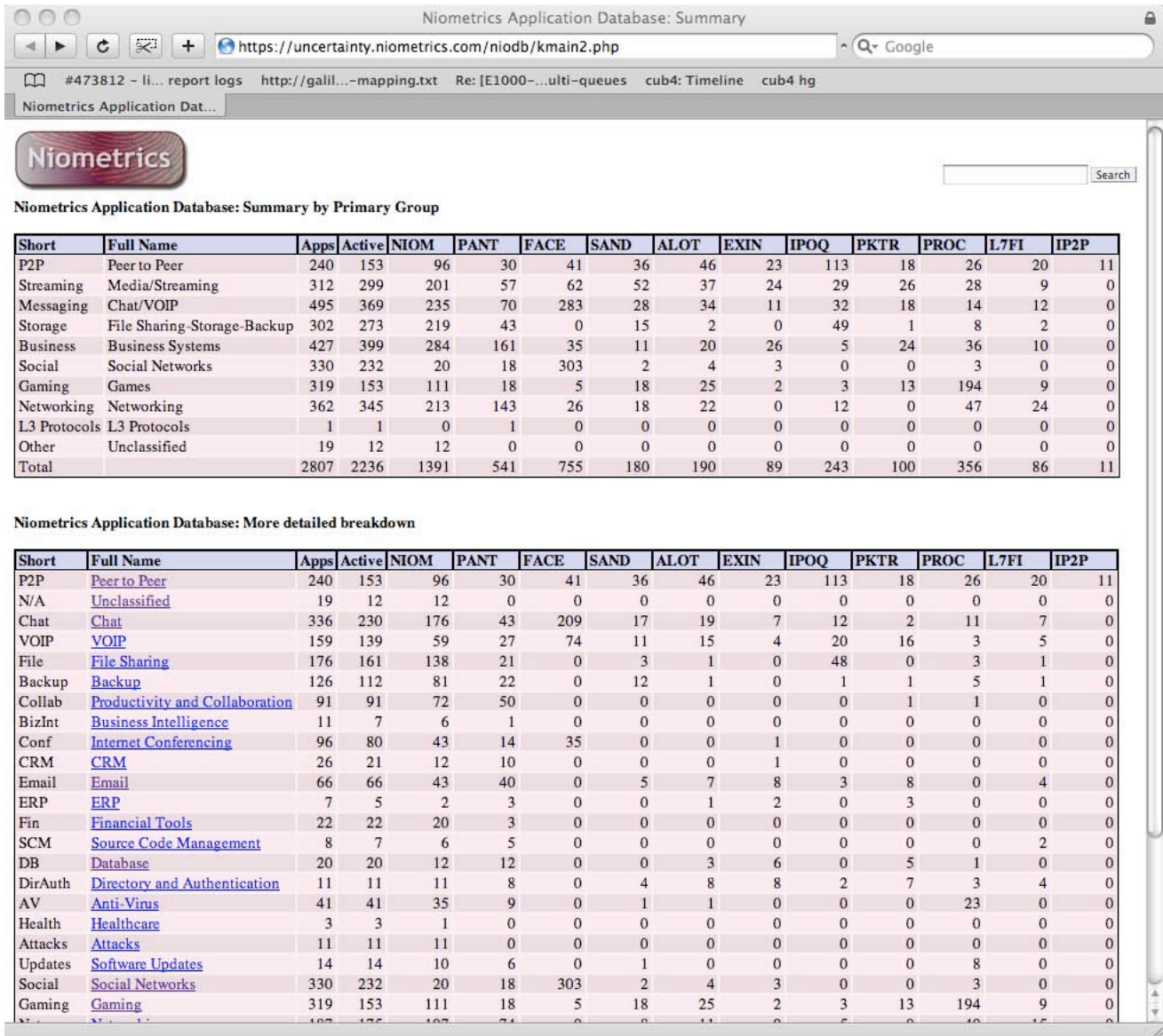
Figure 3: Screenshot of NioDB GUI main screen, showing the application groups and the companies along with the number of applications in each groups that these companies can detect.
