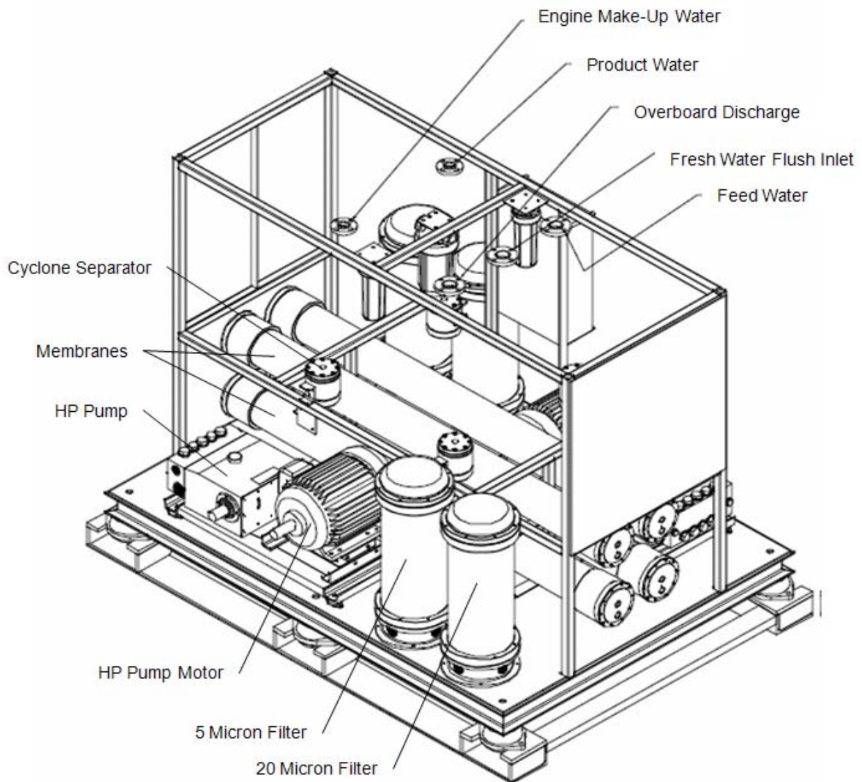
Figure 2-7: RC7000 Plus Reverse Osmosis Unit Layout [14]
