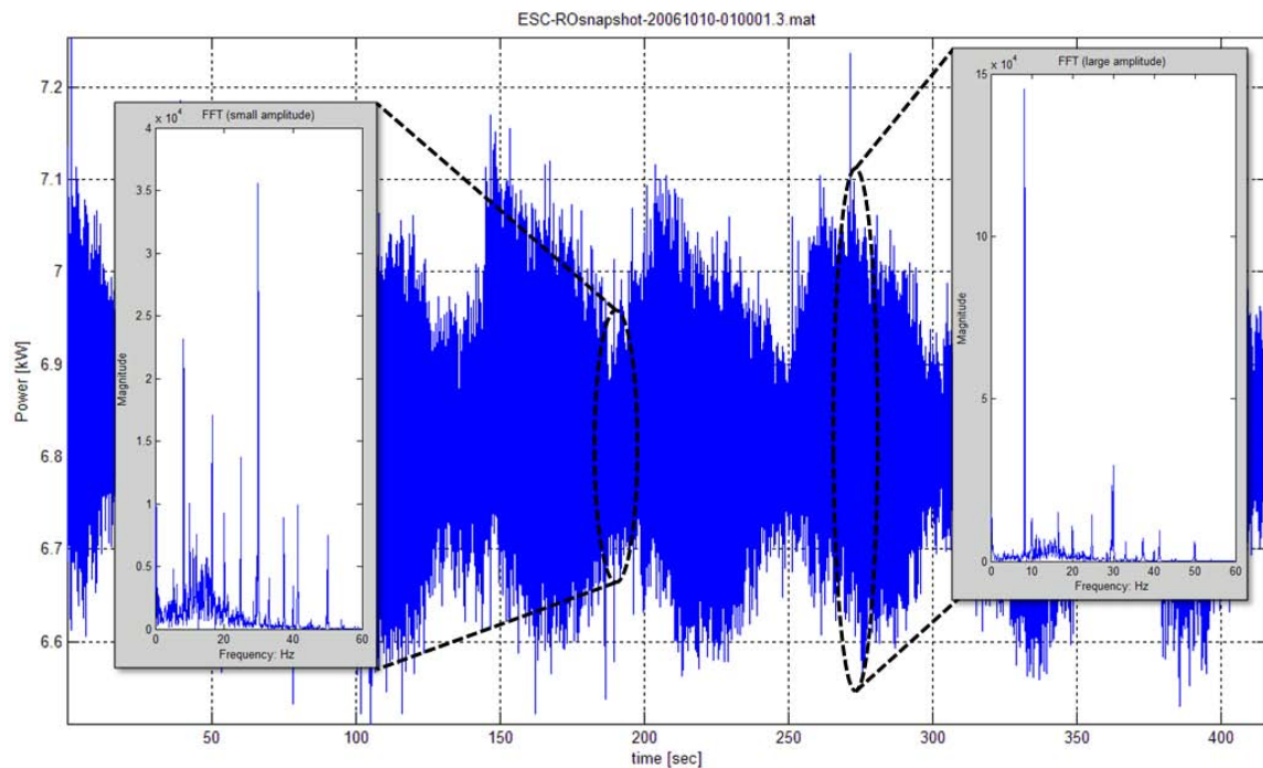
Figure 3-12: Abnormal HP Pump Power Modulation
