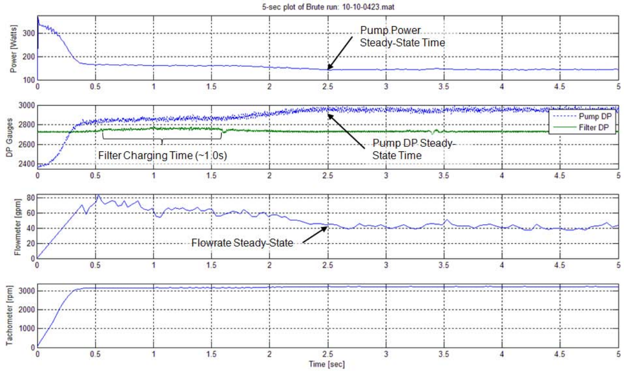
Figure 5-3: Complete Data Set for a Clean Filter Start on the Test Stand
