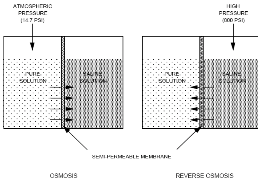
Figure 2-5: The Osmotic System [14]
