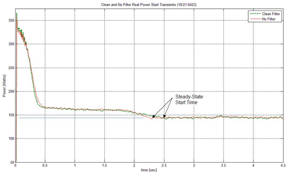
Figure 5-5: Pump Motor Real Power Comparison for Clean and No Filter Conditions
