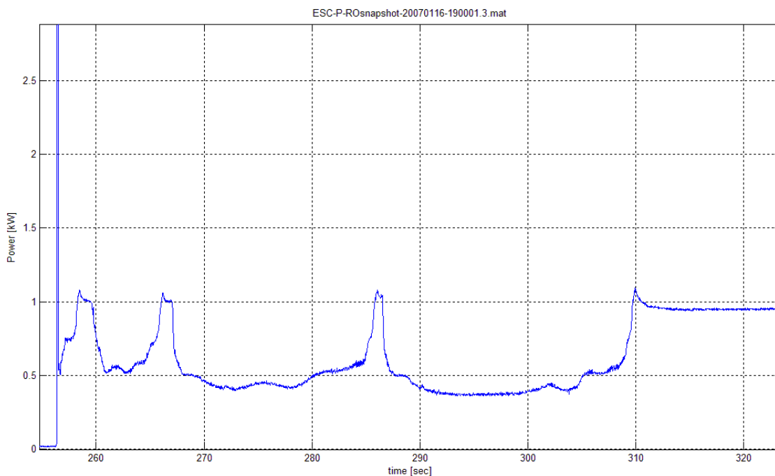
Figure 3-5: An Air Bound LP Pump Start
