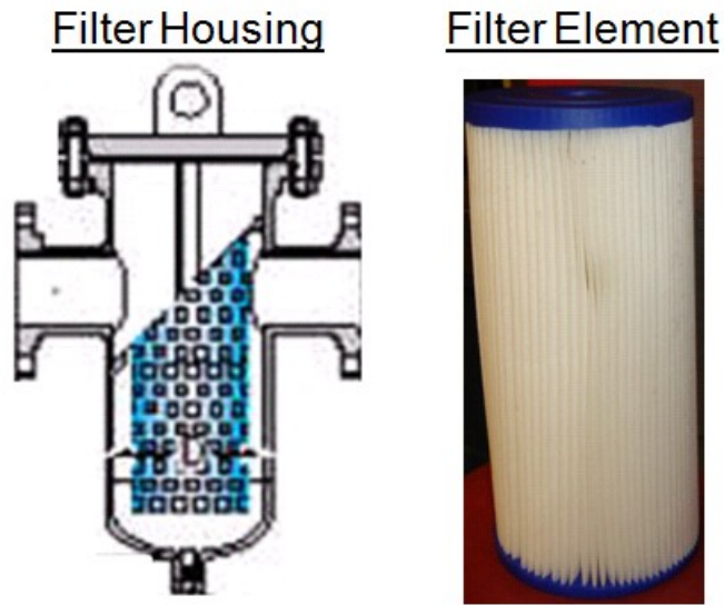
Figure 2-4: Basket Type Filter Housing and Element [13]
