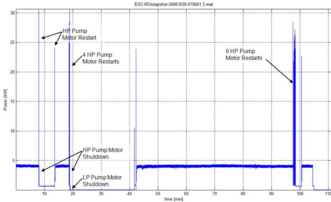
Figure 3-6: Multiple HP Pump Restarts
