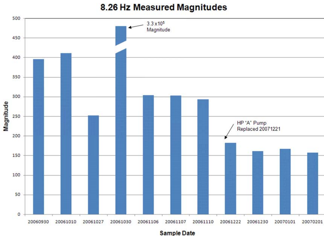
Figure 3-17: 8.26 Hz Magnitude Trending for RO Unit HP Pumps
