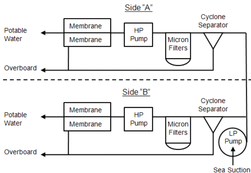
Figure 2-6: Simplified Diagram of the RC7000 Plus RO Unit
