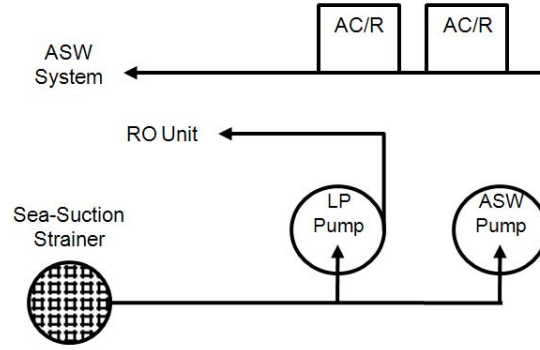
Figure 3-8: RO Unit and ASW Seawater Supply
