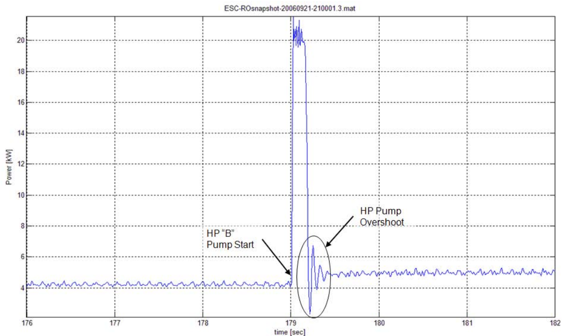
Figure 3-2: Detail of HP "B" Pump Start from Figure 3-1
