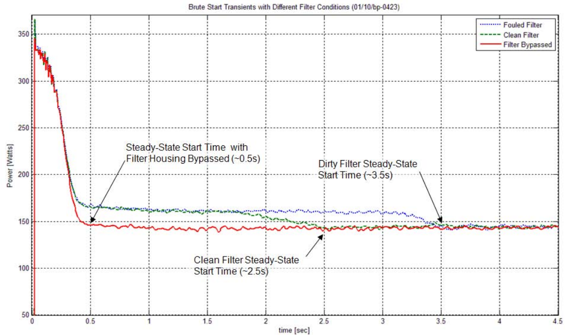
Figure 5-1: Laboratory Test Stand Pump Power Comparison for Various Filter Conditions
