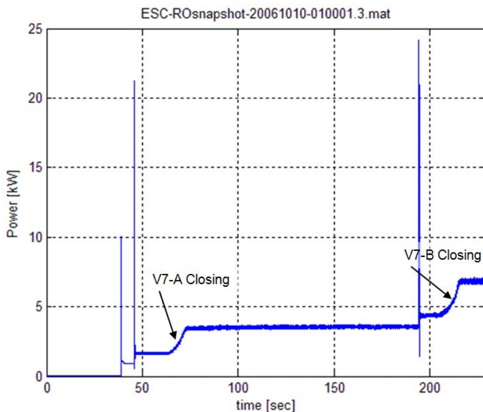
Figure 3-3: RO Unit Major Valve Alignment Changes
