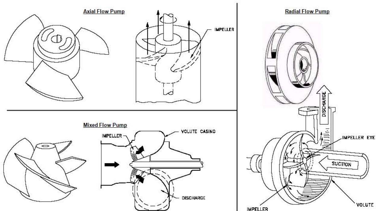
Figure 2-2: Centrifugal Pump Categories with Impeller Details [13]
