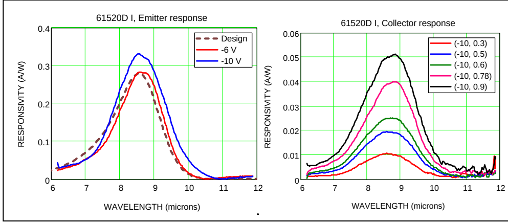
Figure 7. Emitter spectral response at V_E = -6 and -10 V (left panel) and collector response at V_E = -10 V and V_C = 0.3 – 0.9 V (right panel).
