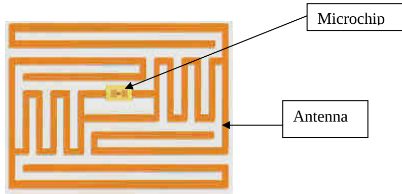
Figure 4 RFID tag
