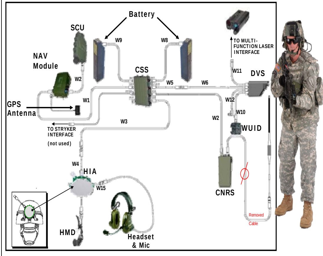
Figure 26. Land Warrior Ensemble (From Witherel, 2008)
