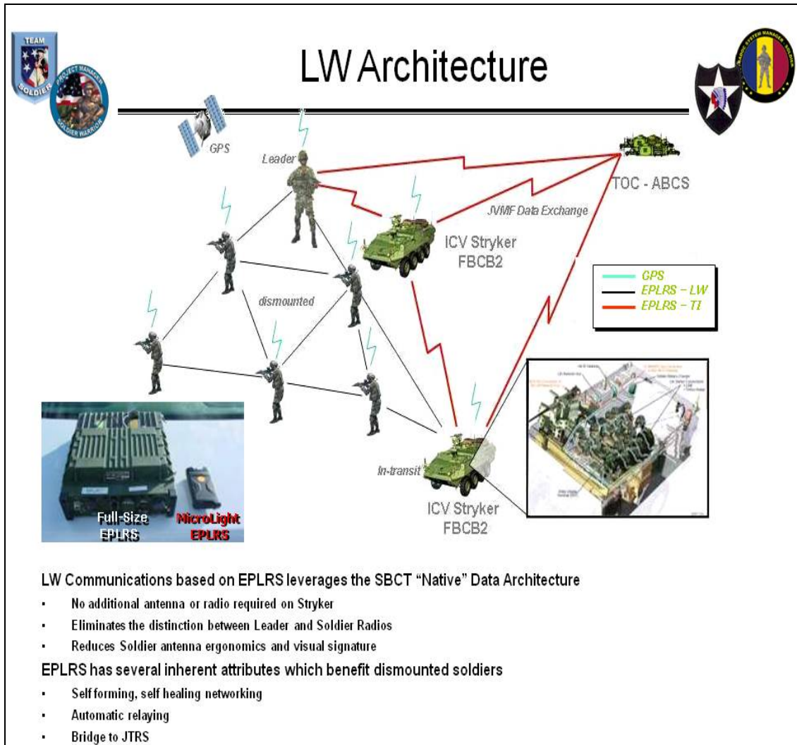
Figure 54. Land Warrior NET Architectural View (From Witherel, 2008)
