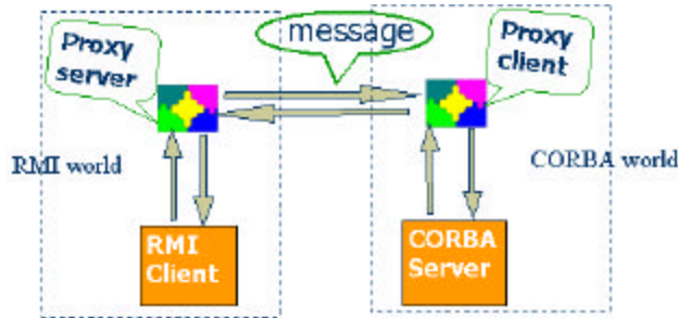
Figure 2. The Interoperation Framework
