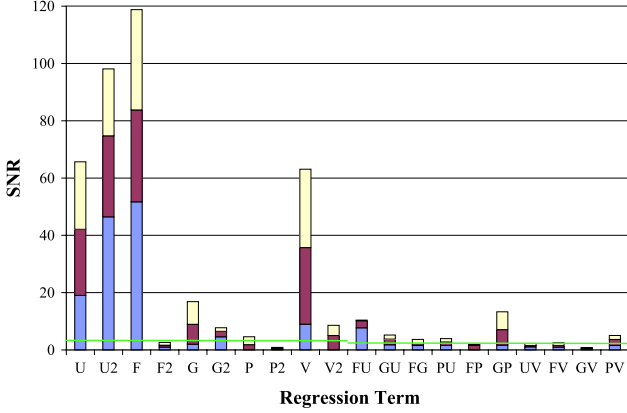
Figure 5: Signal-to-Noise Ratio for Modified Exchange Ratio (Red/Blue + 1)
