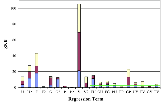
Figure 3: Signal-to-Noise Ratio for Blue Killed
