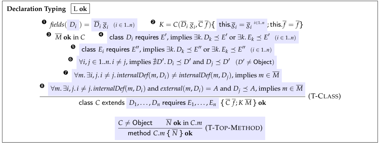
Figure 12: Class and external method typing
