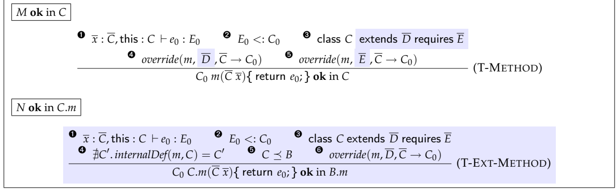
Figure 11: Method typing
