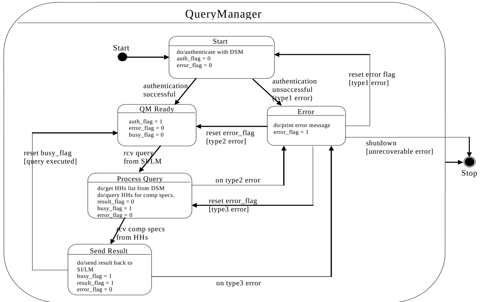
Figure d State Diagram of Query Manager
