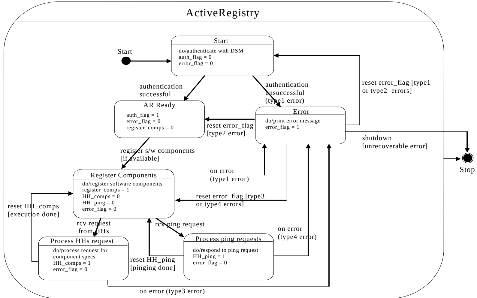
Figure c State Diagram of Active Registry
