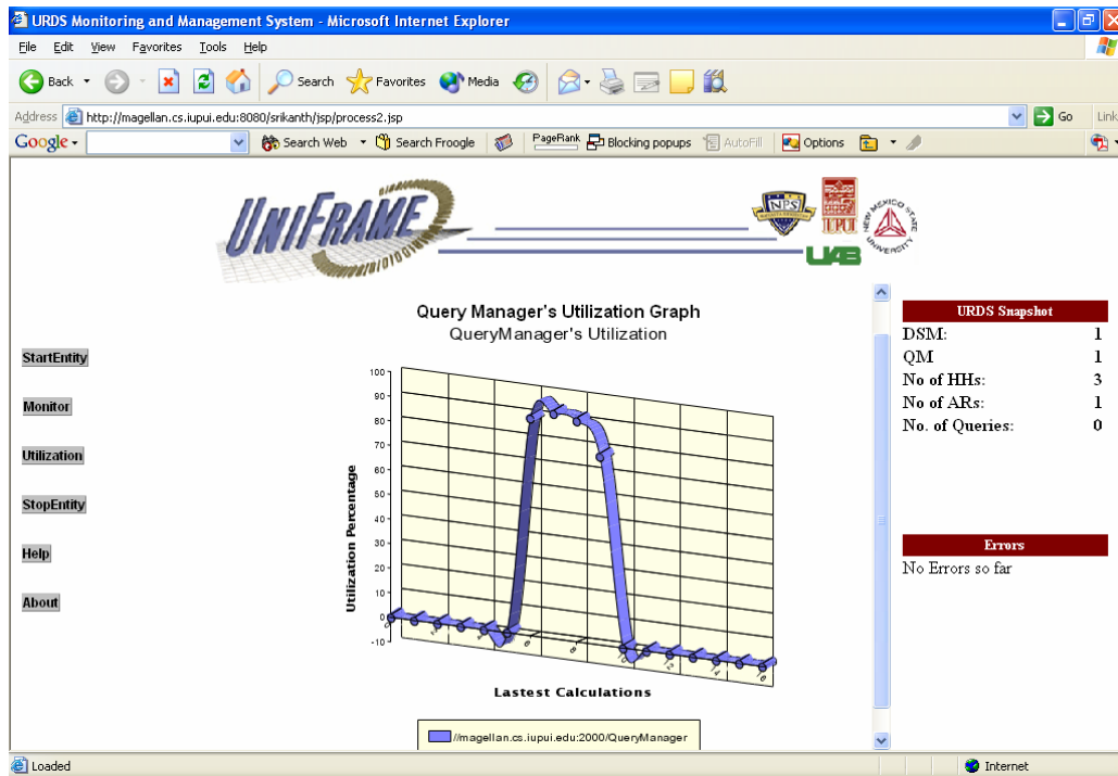
Figure ix: View showing the graph of Query Manager's utilization
