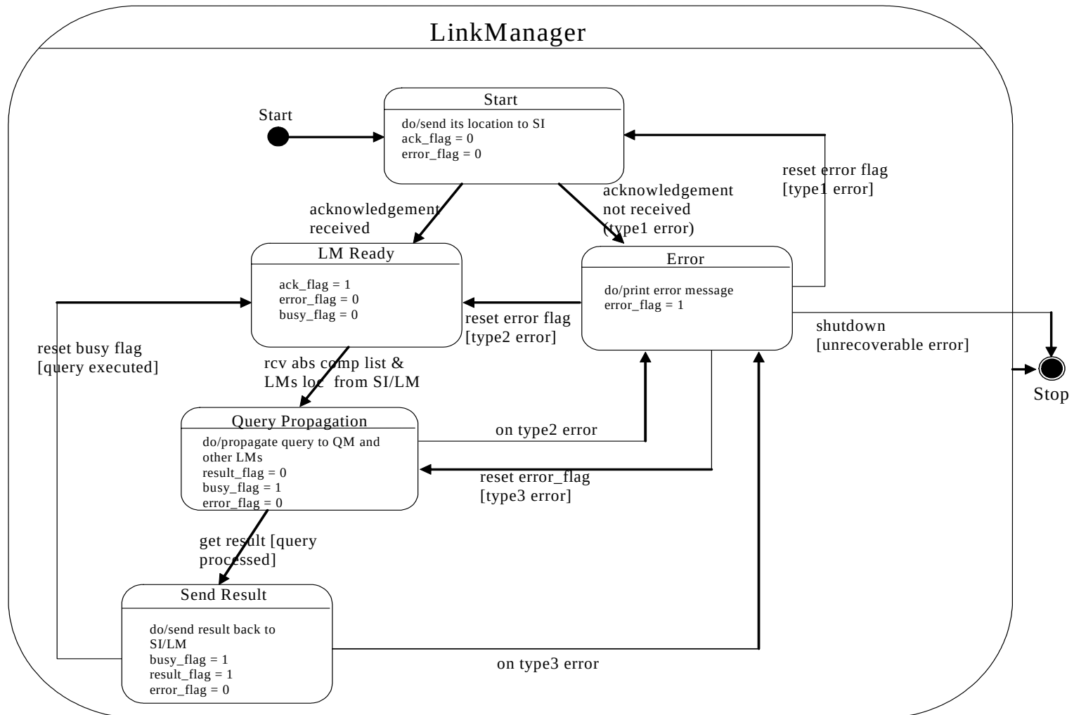
Figure e State Diagram of Link Manager
