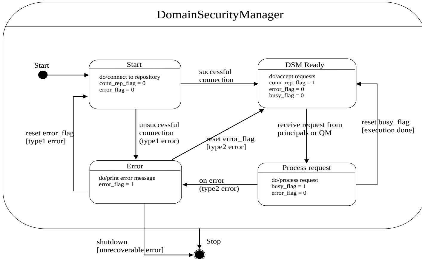
Figure a State Diagram of Domain Security Manager
