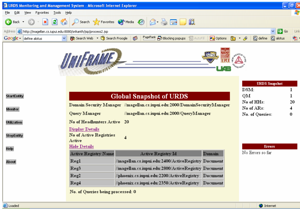
Figure vii: View showing the details of Active Registries
