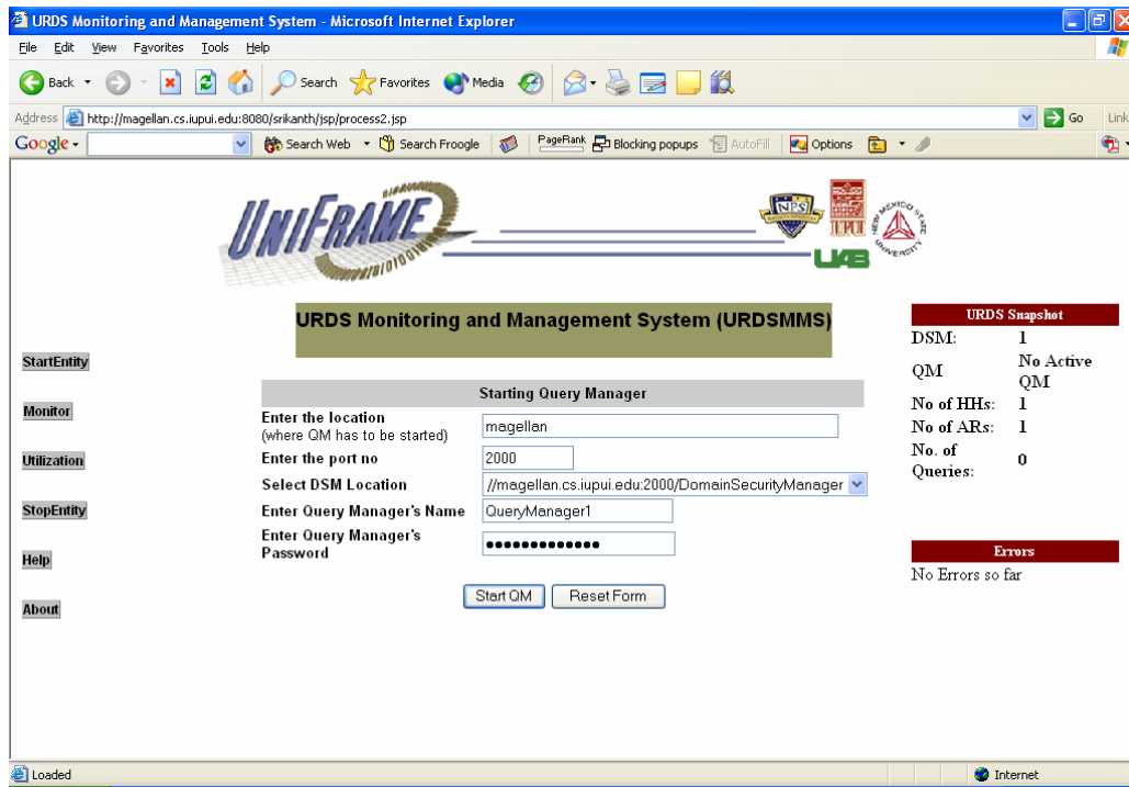
Figure v: View showing the initiation of a Query Manager
