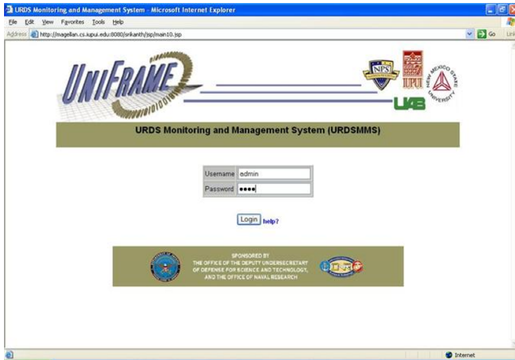
Figure 4.6 main.jsp view
