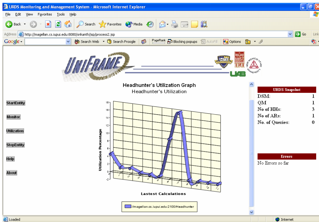
Figure viii: View showing the graph of Headhunter's utilization
