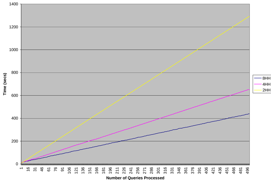
Figure 5.7 Comparison of number of queries processed for different sets of Headhunters
