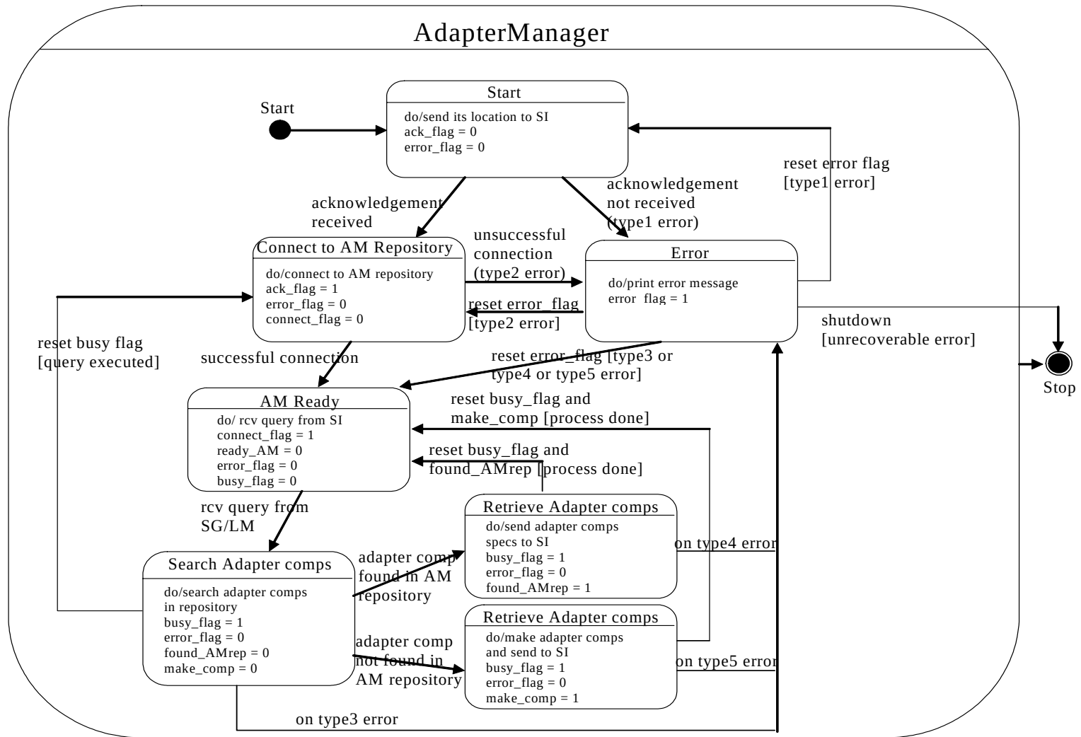
Figure f State Diagram of Adapter Manager
