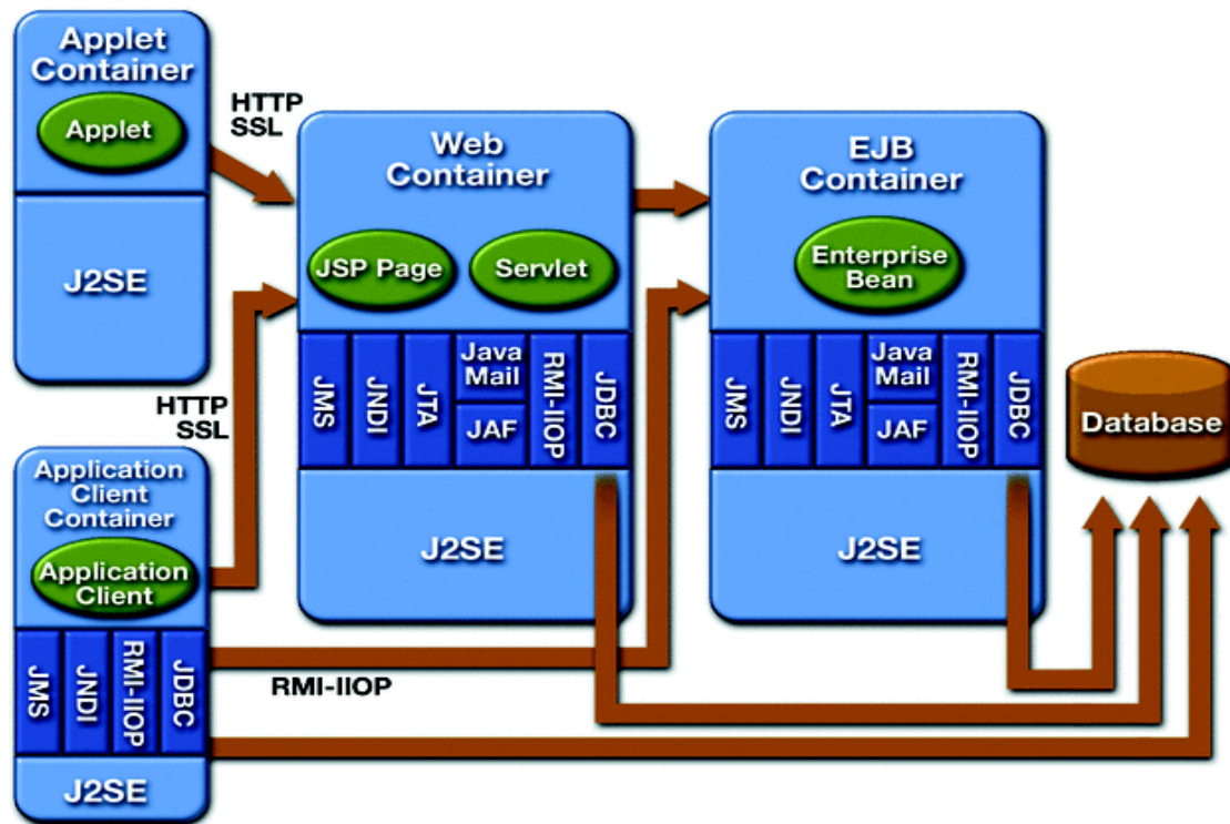
Figure 4.4 Components and Containers of J2EE Model. [SUN01a]
