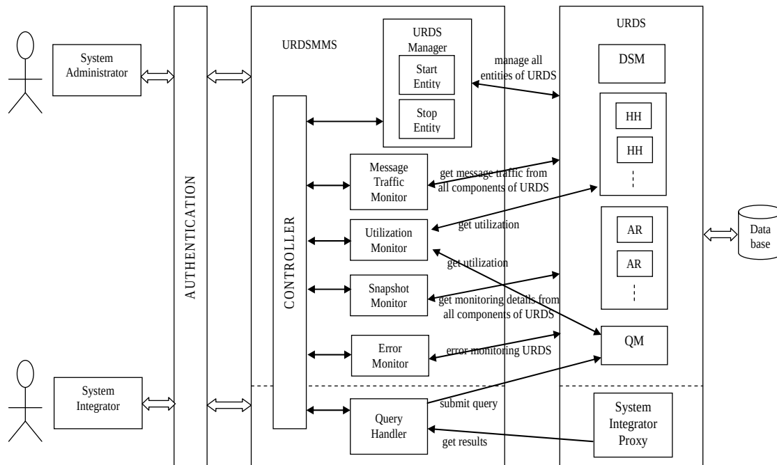
Figure 4.1: URDS Monitoring and Management System Architecture
