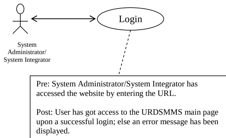
Figure 4.2 Use Case Diagram for a successful/unsuccessful login
