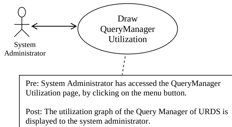
Figure vi Use Case Diagram for display of Query Manager Utilization graph
