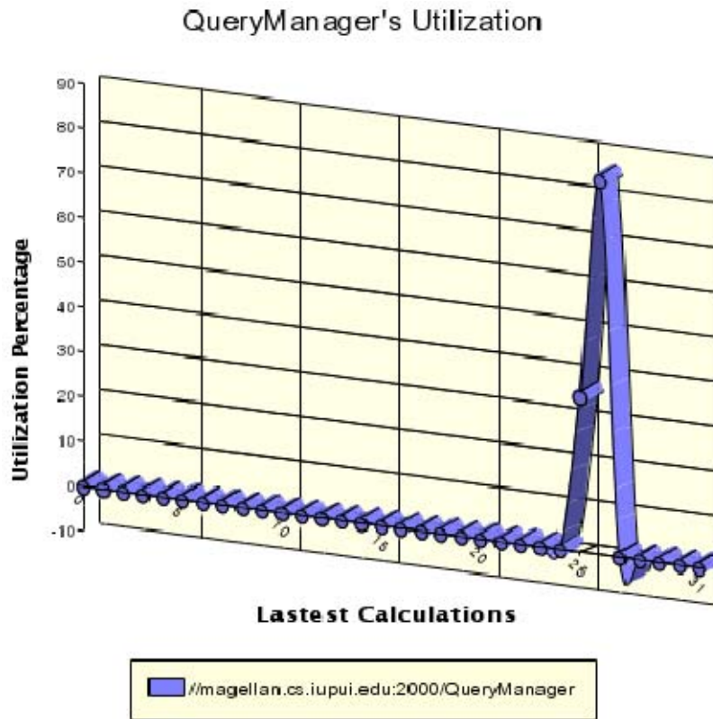
Figure 5.3 Utilization of Query Manager
