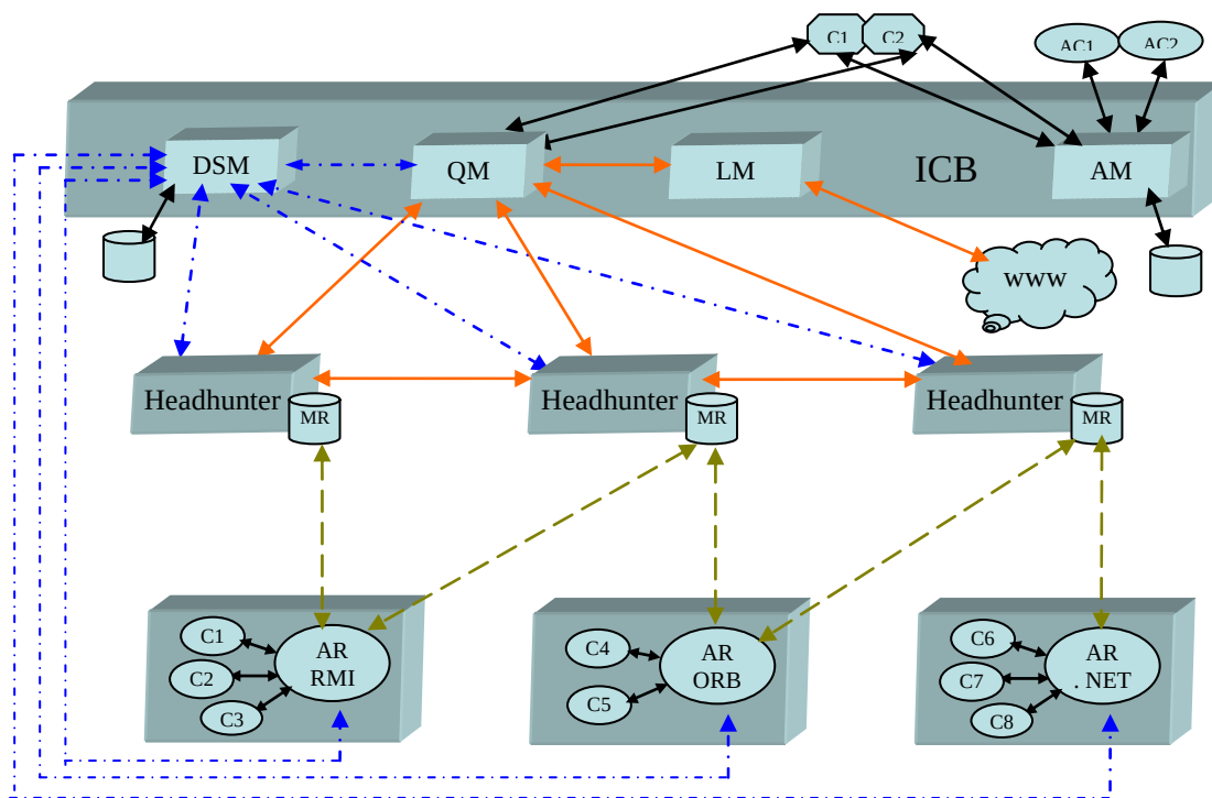
Figure 2.2. URDS Architecture [DEV05]
