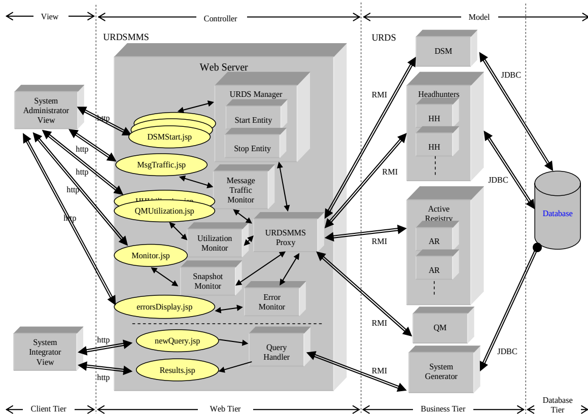
Figure 4.5 URDSMMS Implementation
