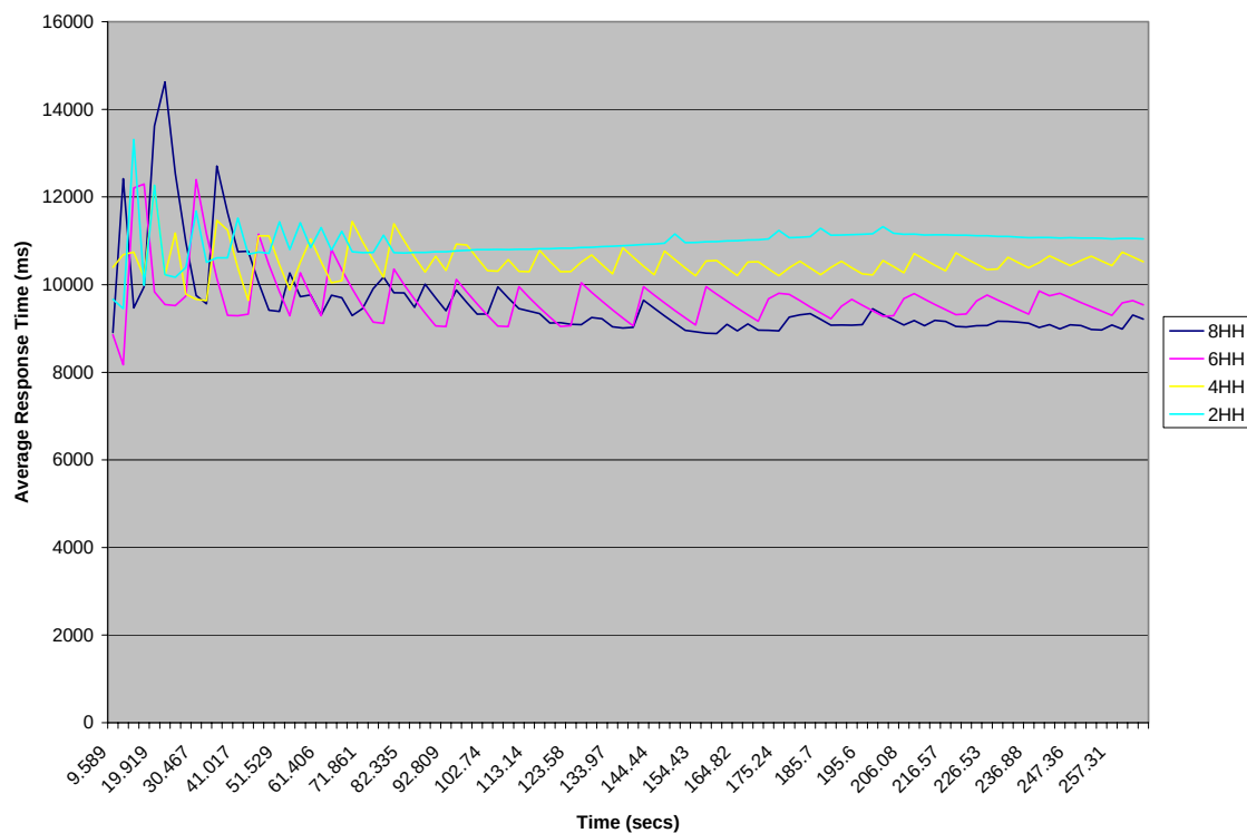
Figure 5.6 Comparison of average response times for different sets of Headhunters (enlarged version)
