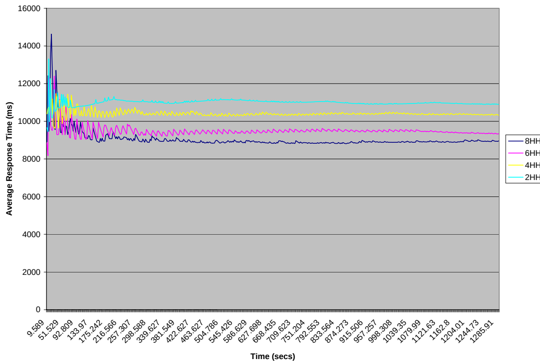
Figure 5.5 Comparison of average response times for different sets of Headhunters
