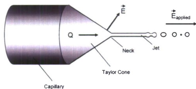
Figure 2. Schematic representation of an electro spray in the cone-jet regime (see Figure 1 for V \approx V_c ). E represents the surface normal electric field and Q is the volume flow rate. Note the varicose wave on the surface of the jet. The electric field at the neck ( E ) and the external field ( E_{\text{applied}} ) are denoted. In the mixed ion-droplet regime (see the middle configuration in the bottom row of Figure 1) the ejected spray consists of a mixture of droplets and ions (the latter not shown here).
