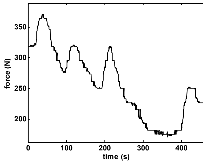
Figure 19: Extrusion force for part in Figure 18 fabricated with a constant ram velocity of 10 \mu\text{m/s} .
