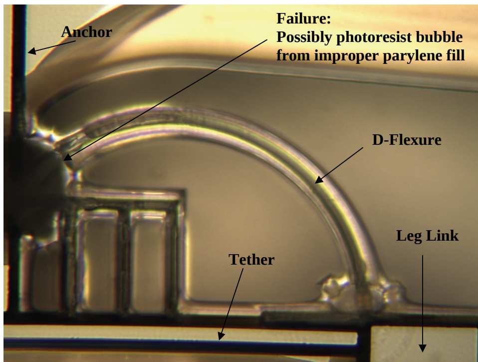
Figure 5. This photograph from the optical microscope illustrates a failure at the junction between the D-flexure and the anchor, possibly from improper parylene fill or photoresist bubbles.
