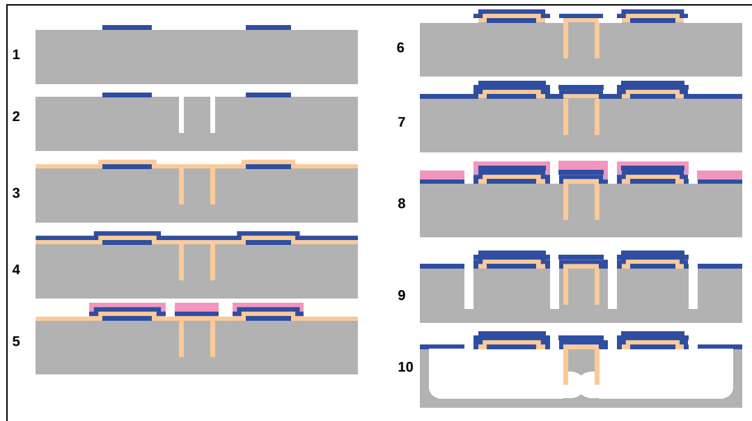
Figure 2. Parylene fabrication process: 1. Pattern (dummy) actuators; 2. Etch deep trenches; 3. Coat parylene; 4. Deposit oxide hard mask; 5. Pattern photoresist for parylene etch; 6. Etch parylene and photoresist; 7. Deposit additional oxide; 8. Pattern oxide, thin photoresist; 9. Etch deep trenches; and 10. \text{XeF}_2 release.
