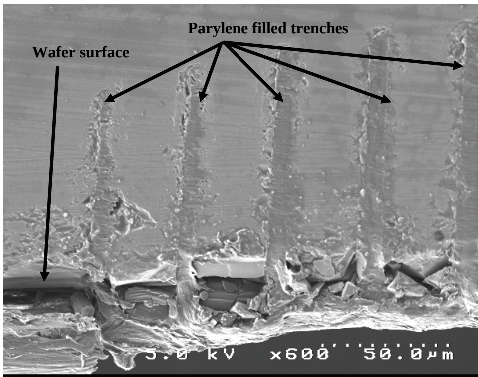
Figure 10. This photograph from the SEM shows the parylene filled trenches of widths of 3, 4, 5, 6, and 7 \mu\text{m} spaced 30 \mu\text{m} apart. The etch depth is approximately 76 \mu\text{m} for the 5 \mu\text{m} wide trench.
