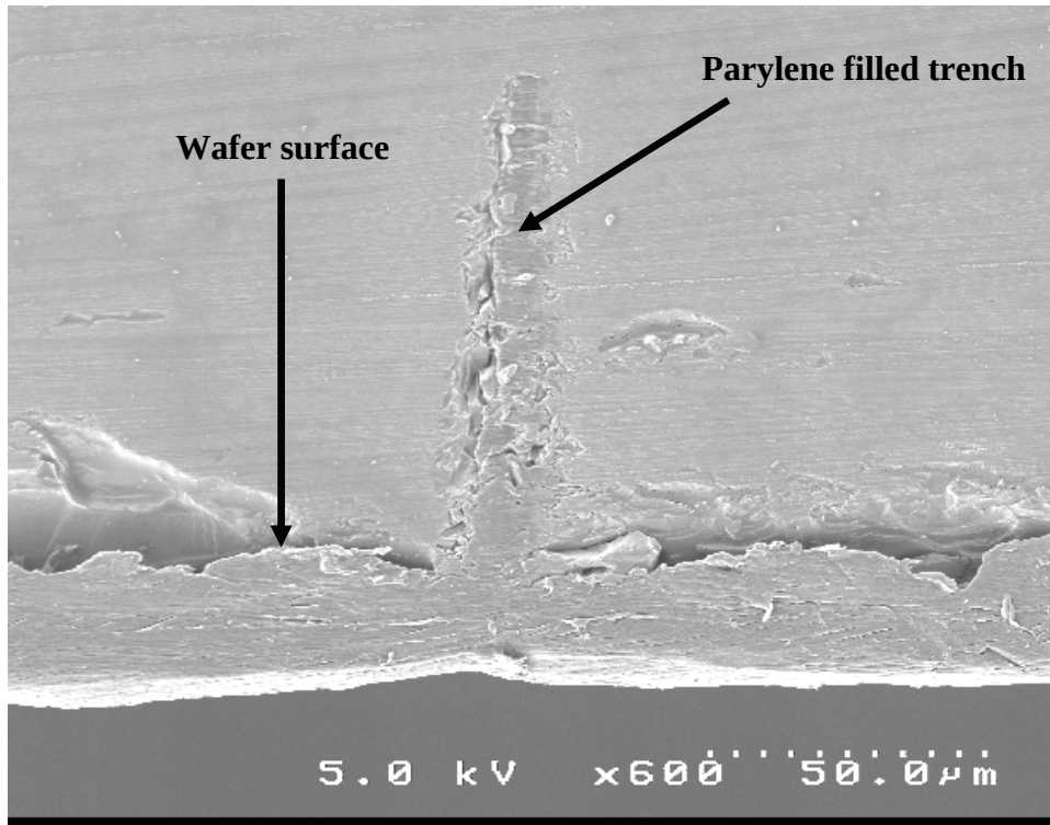
Figure 9. This photograph from the SEM shows a parylene filled trench 5 \mu\text{m} wide. The etch depth here is approximately 82 \mu\text{m} .
