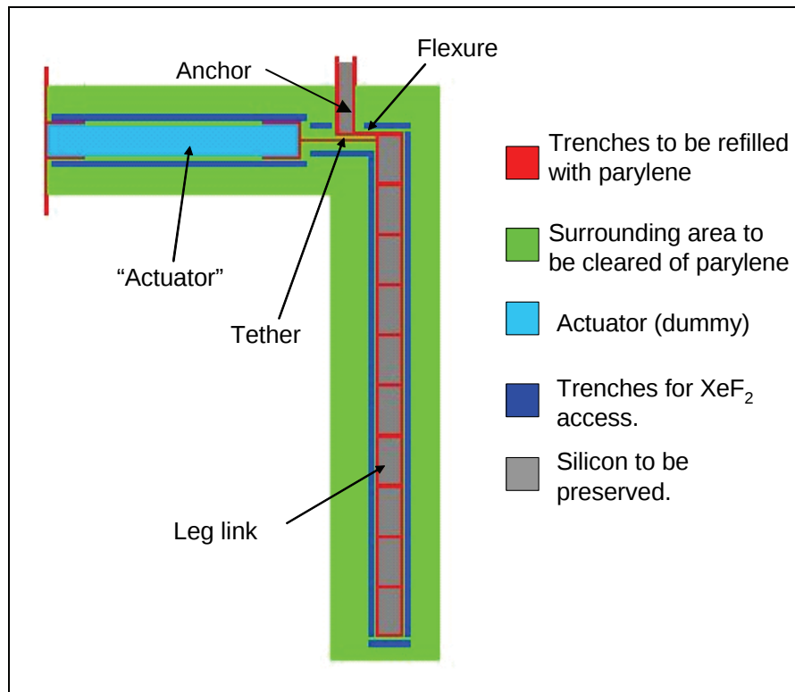
Figure 3. The sample actuator/flexure/leg-link test structure. In figures 4–8 the structures also contain a D-Flexure in parallel to the flexure.
