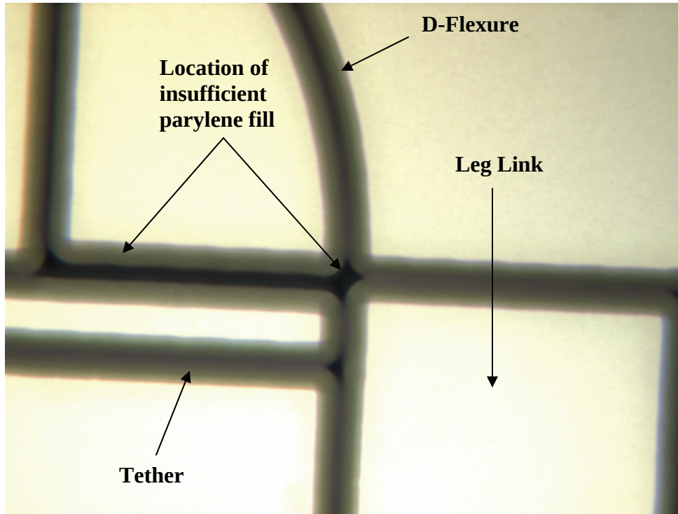
Figure 7. This photograph from the optical microscope shows insufficient parylene fill in the dark black areas near the D-Flexure-leg link four-trench junction.
