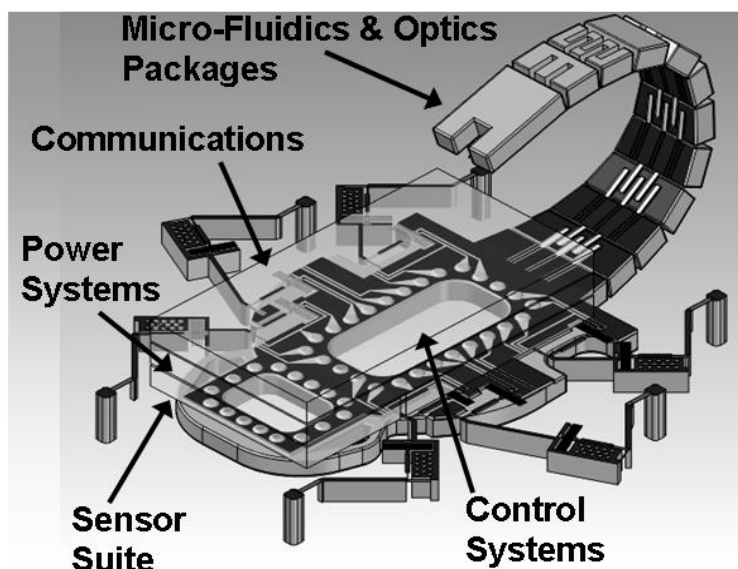
Figure 1. The conceptual design of the ground mobile millimeter-scale robot highlighting various components and systems required for operation.
