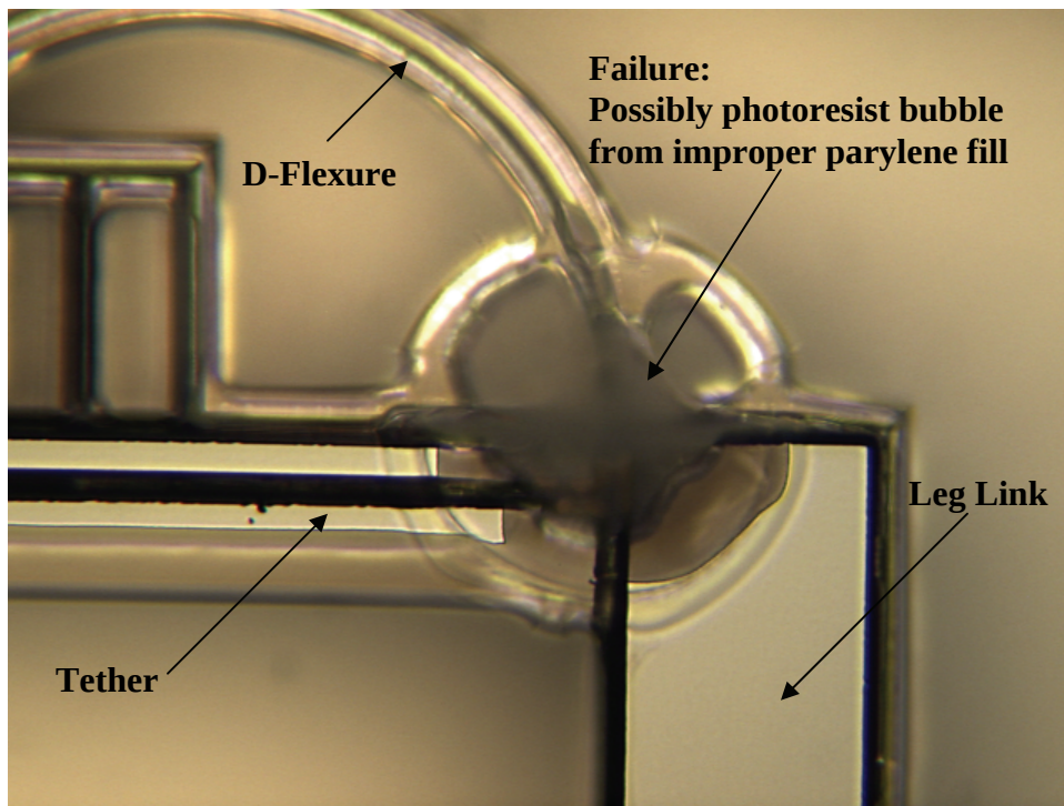
Figure 4. This photograph from the optical microscope illustrates failure at the junction between the flexure and the leg link, possibly from improper parylene fill or photoresist bubbles.
