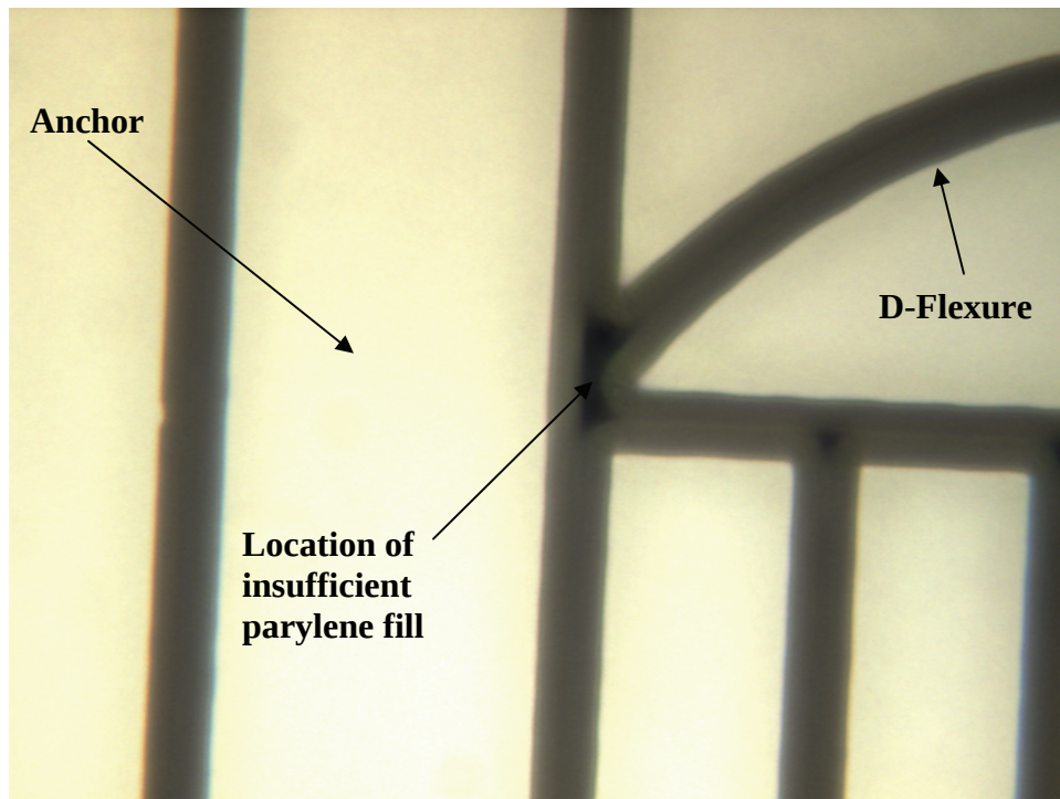
Figure 6. This photograph from the optical microscope shows insufficient parylene fill in the dark black areas near the four-trench junction at the anchor and D-Flexure intersection.
