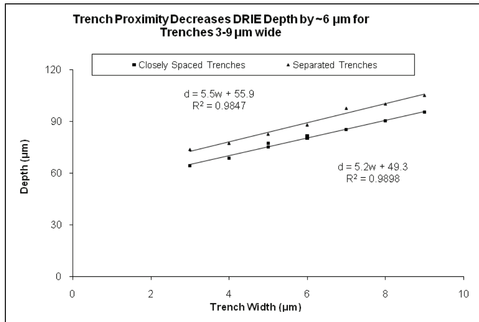
Figure 11. The graph shows that trenches that are close together result in more shallow etch profiles and that trench depth is linearly dependent on trench width within the range of etch.
