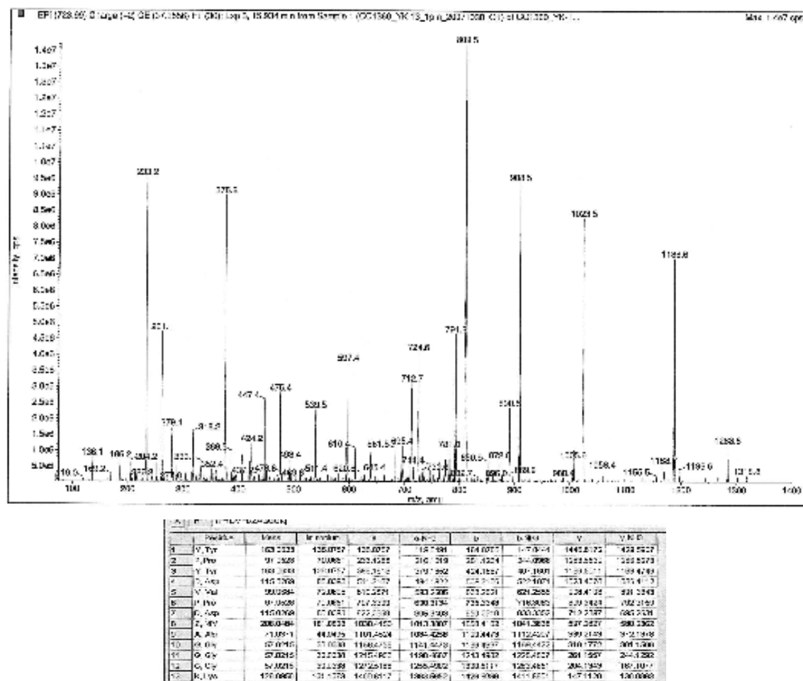
Fig 3. We synthesized a 13 mer, NT containing peptide (YPDYDPD-NT-AGGGK) and examined it by tandem mass spec to identify its sequence. The MS/MS mass spectrum clearly demonstrates the detection and location of the nitrated tyrosine. The peptide gives a strong signal by EMS and a strong y ion series in the MS/MS fragmentation patterns thus validating this methodology for the identification of NT containing peptides.
