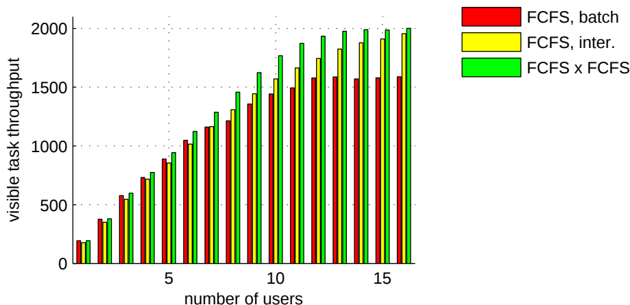
Figure 6.14: The effect of the number of users on batchactive usage of \text{FCFS} \times \text{FCFS} , interactive usage of FCFS, and batch usage of FCFS for visible task throughput. Visible task throughput is the number of needed tasks that have executed; i.e., the number of tasks whose outputs were needed which were delivered to their submitting users. Higher visible task throughput is better. Visible throughput is shown to illustrate that it does not worsen as metrics such as mean visible response time improve. Improving visible throughput is not a goal in itself. A server is concerned with billable resources, which includes resources used by needed and unneeded tasks (and fractions thereof) under the non-speculative pricing mechanism. \text{FCFS} \times \text{FCFS} provides the best visible task throughput.
