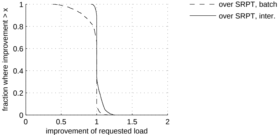
Figure 6.54: Improvement of batchactive usage of SRPT \times FCFS over interactive and batch usage of SRPT for requested load. Requested load is the server busy time charged to the user. The horizontal axis shows improvement factors while the vertical axis indicates the fraction of the runs in which the improvement was at least as much indicated on the horizontal axis. Better batchactive performance is reflected by the area under the curves for improvement values greater than 1, while worse batchactive performance is reflected by the area above the curves for improvement values less than 1. Data along the line where improvement equals 1 reflects equal performance for some user and task characteristics. SRPT \times FCFS provides better requested load than interactive SRPT and worse requested load than batch SRPT . Doing worse against batch FCFS is expected and was explained in Chapter 6.2.2. The arithmetic mean improvement is 1.020 over interactive SRPT and 0.956 over batch SRPT. (A mean improvement factor less than 1 is overall worse performance.)
