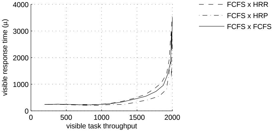
Figure 6.38: The relationship on batchactive usage of \text{FCFS} \times \text{HRR} , batchactive usage of \text{FCFS} \times \text{HRP} , and batchactive usage of \text{FCFS} \times \text{FCFS} between visible throughput and visible response time as the number of users was varied from 1 to 16 and other parameters were held constant. Both axes are dependent axes; the horizontal axis indicates visible throughput while the vertical axis indicates mean visible response time. \text{FCFS} \times \text{HRP} provides better visible task throughput while simultaneously providing better mean visible response time.
