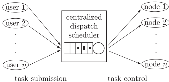
Figure 1.2: Centralized cluster scheduler. Users send task requests and cancelations to a centralized cluster scheduler. This scheduler orders and distributes work among multiple cluster nodes. Task outputs are written to a shared store (not shown) accessible by the submitting user.
