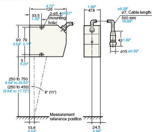
Figure 6c. Keyence LK-503
