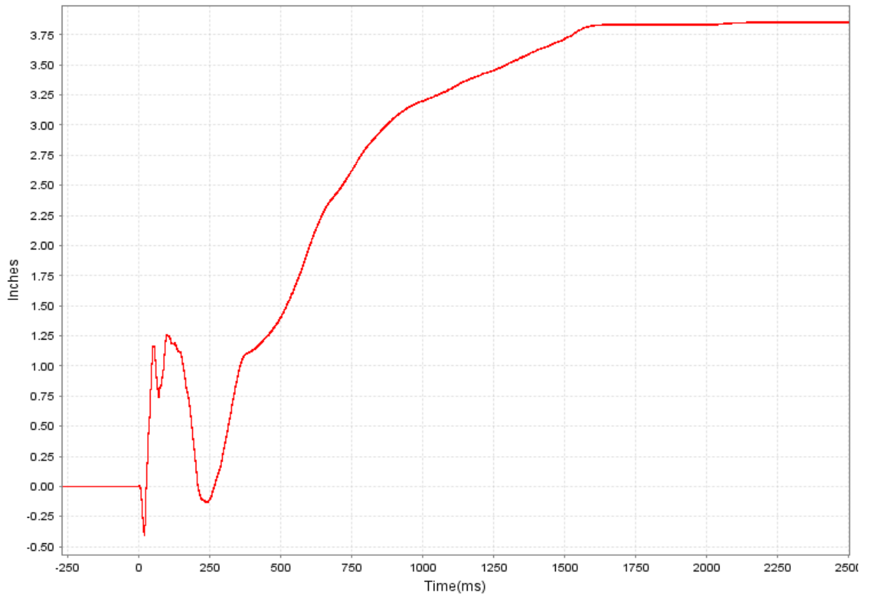
Figure 9. Output from a Celesco PT101 Series Cable Extension Transducer. The record shows motion of a hydraulically adjustable seat as the hydraulic system is breached.
