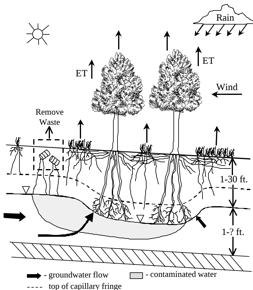
Figure 1. Cross-section through a Phytostabilization Site
