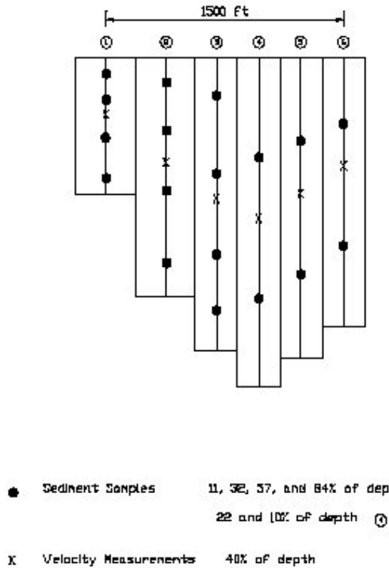
Figure 2.1 The USACE Vicksburg District suspended-sediment sampling routine
