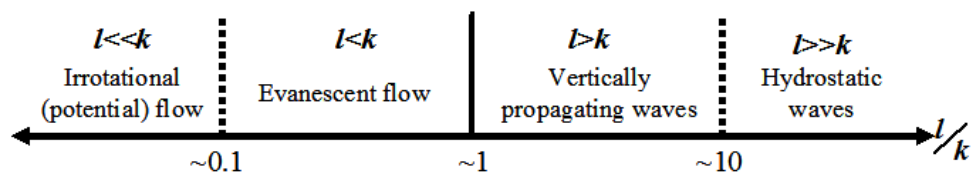
Figure 1.2: Spectrum of mountain wave regimes as a function of the ratio of Scorer parameter to wave number. Adapted from Lin (2007).
