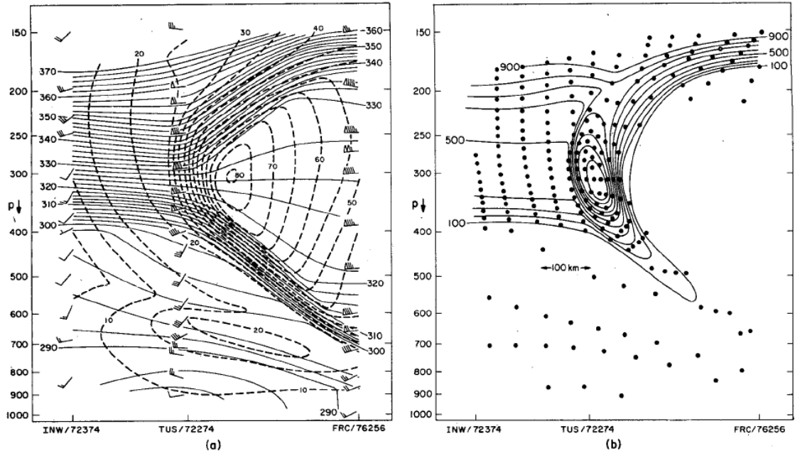
Figure 1.8: Cross-section of (a) potential temperature (solid, K), wind speed (dashed, \text{ms}^{-1} ), and wind barbs ( \text{ms}^{-1} ) and (b) potential vorticity ( 10^{-7} \text{Kmb}^{-1}\text{s}^{-1} ) valid 0000 UTC 17 April 1976. Vertical coordinate is pressure in mb, and data from rawinsonde soundings launched from Winslow, AZ (INW), Tucson, AZ, and Fraccionamiento, Mexico (FRC). From Shapiro (1981).
