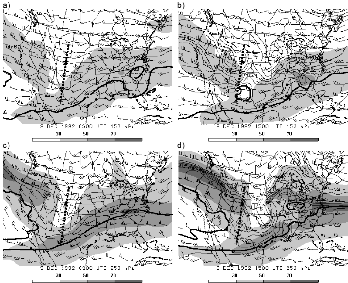
Figure 2.5: Wind speed ( \text{ms}^{-1} , shaded) and potential vorticity (PVU, or 10^{-6} \text{Km}^2\text{s}^{-1}\text{kg}^{-1} ) at (a-b) 150 hPa and (c-d) 250 hPa at 0300 UTC (left column) and 1500 UTC 9 December 1992 (right column). Data from NCEP/NCAR North American Regional Reanalysis. Dynamic tropopause (2 PVU) depicted by bold contour. Data was smoothed with six passes of a Gaussian filter to eliminate noise after winds were corrected from model-relative to true. Cross-section for Fig. 2.6 denoted by dotted line. Aircraft incident location denoted by star.
