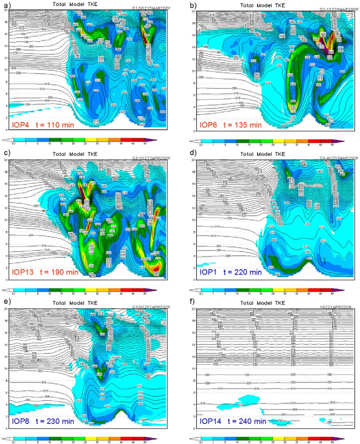
Figure 4.21: Model-parameterized TKE (shaded, m^2s^{-2} ) and potential temperature (contoured, K) for the IOPs and times indicated (representing the time of maximum TKE above the tropopause). Red text in the caption denotes strong stratospheric wave IOPs and red text denotes weaker stratospheric wave IOPs.
