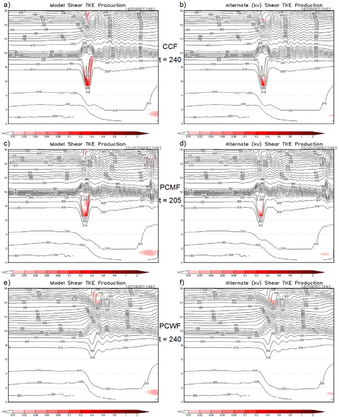
Figure 4.14: Model-parameterized mechanical shear TKE production (left, shaded, m^2 s^{-3} ) from Eq. (4.2) and alternate mechanical shear TKE production (right, shaded, m^2 s^{-3} ) from Eq. (4.7). Output shown at time of maximum TKE for (a-b) CCF (240 min), (c-d) PCMF (205 min), and (e-f) PCWF (240 min) simulations.
