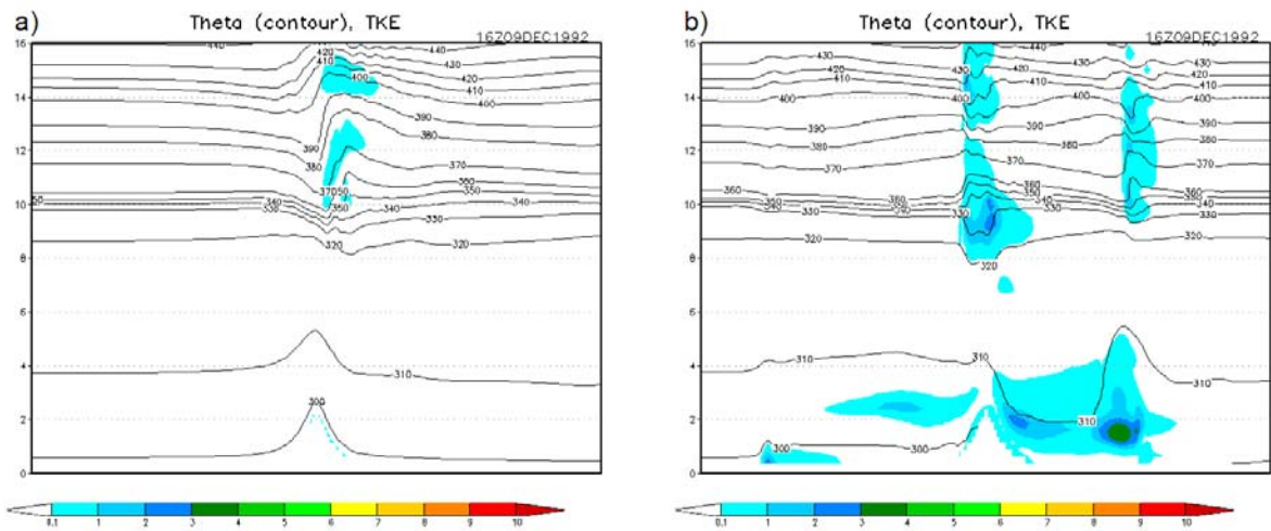
Figure 4.8: Same as Fig. 4.7, except for (a) PCU and (b) PCNS simulations.
