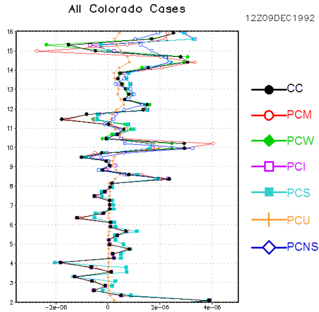
Figure 4.9: Scorer parameter ( \text{m}^{-2} ) in the 2 to 16 km AGL layer associated with the upstream boundary conditions for all 9 December 1992 Colorado simulations as indicated.
