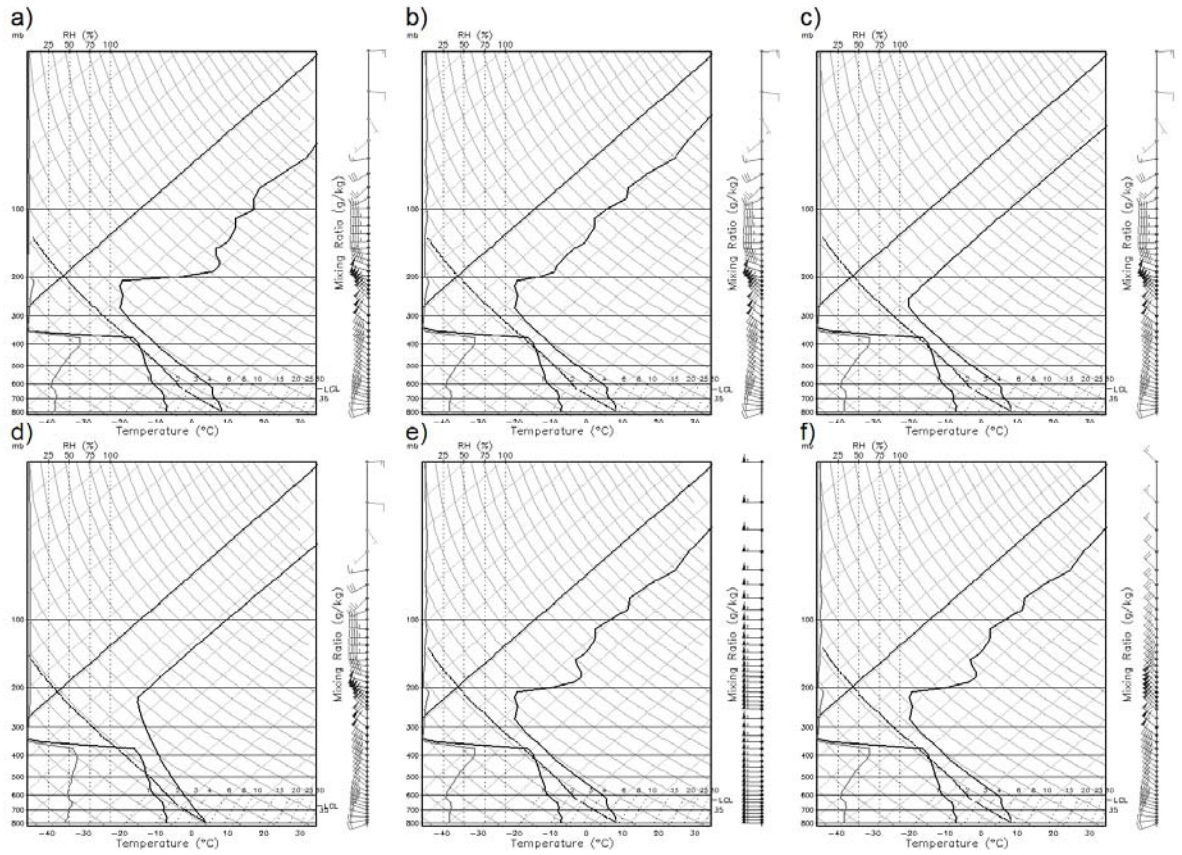
Figure 4.2: Initialization soundings of temperature, dew point, and winds for simulations (a) PCM, (b) PCW, (c) PCI, (d) PCS, (e) PCU, and (f) PCNS. Simulation designations described in Table 4.1
