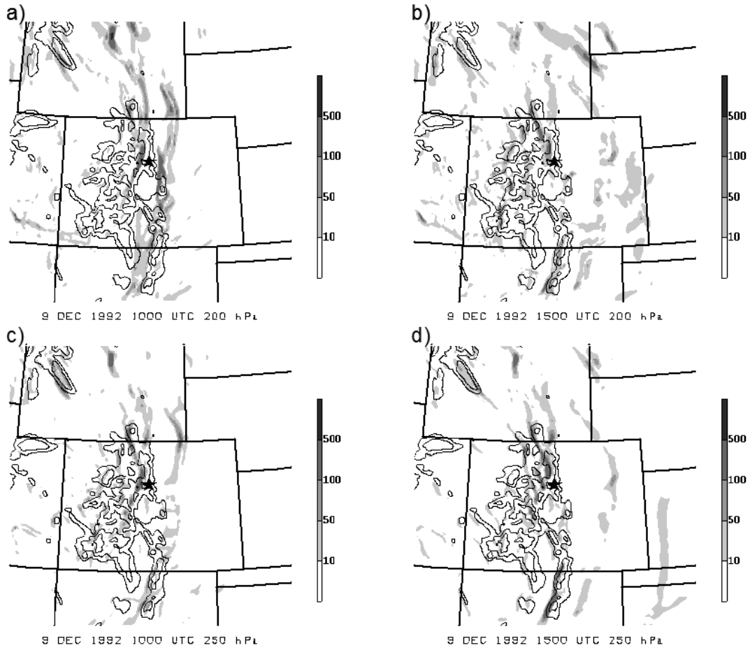
Figure A.7: Simulated 200 hPa GEMPAK-derived horizontal frontogenesis function ( K 100 \text{ km}^{-1} 3\text{hr}^{-1} , shaded) at (a) 1000 UTC and (b) 1500 UTC and at 250 hPa at (c) 1000 UTC and (d) 1500 UTC 9 December 1992. Terrain contours at 2.5,3, and 3.5 km. From 6 km NHMASS full-terrain simulation. Aircraft accident location denoted by star.
