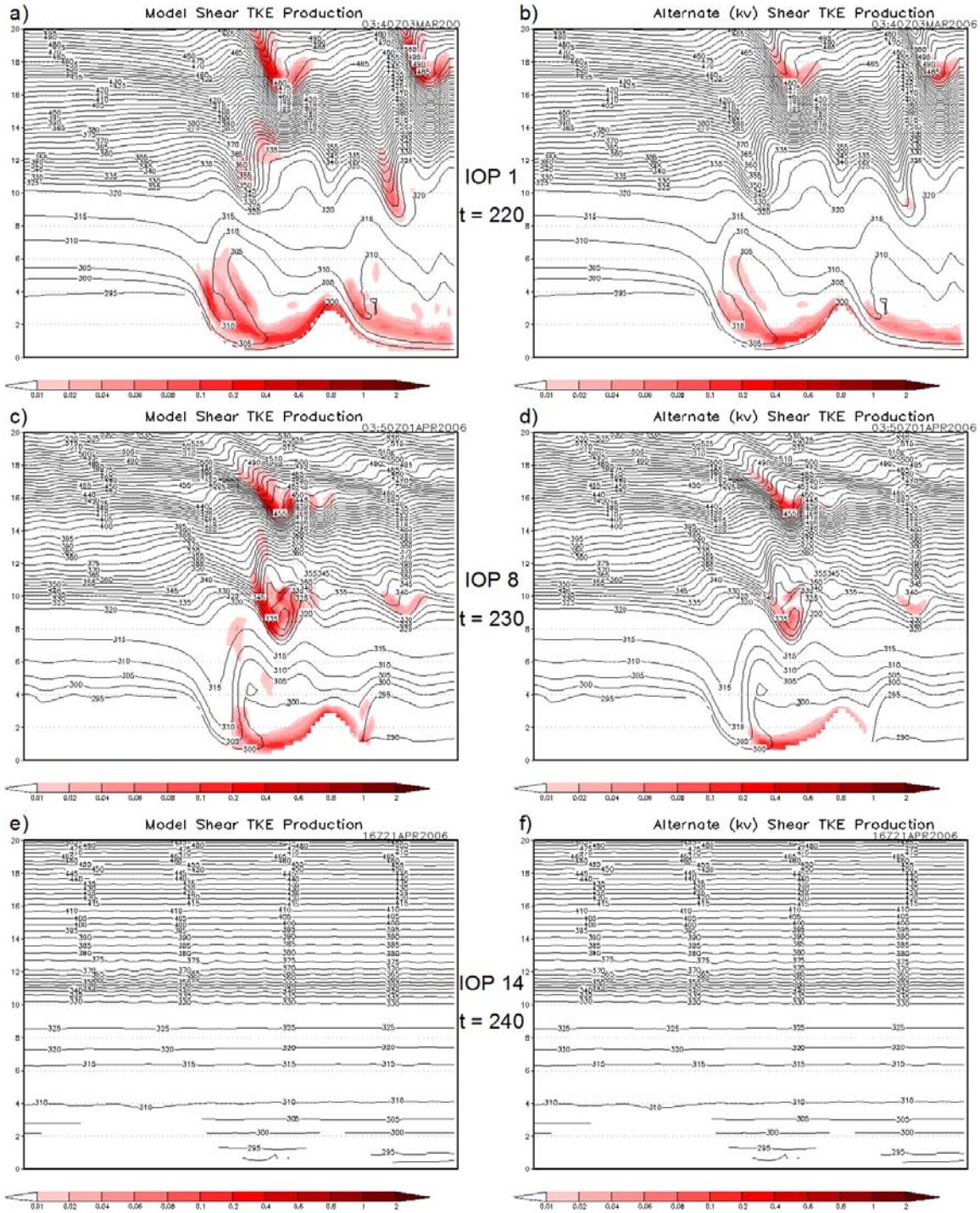
Figure 4.23: Model-parameterized mechanical shear TKE production (left, shaded, m^2s^{-3} ) from Eq. (4.2) and alternate mechanical shear TKE production (right, shaded, m^2s^{-3} ) from Eq. (4.7). Output shown at time of maximum stratospheric TKE for the three weak stratospheric wave cases.
