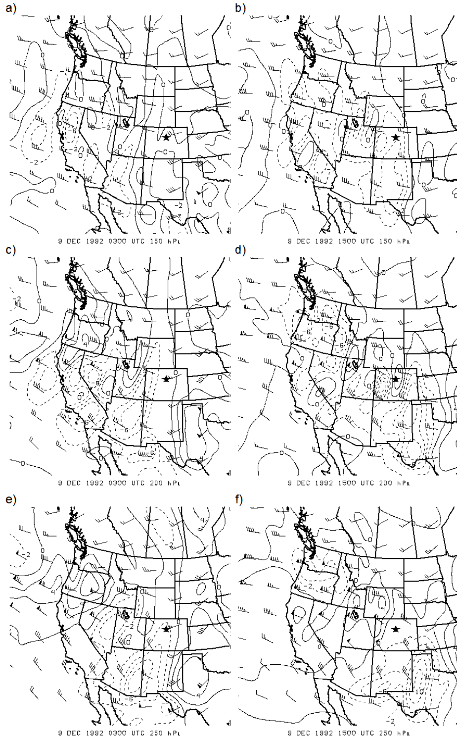
Figure 2.8: Temperature advection ( \text{Ks}^{-1} \times 10^{-4} ) and winds ( \text{ms}^{-1} ) at (a-b) 150 hPa, (c-d) 200 hPa, and (e-f) 250 hPa at 0300 UTC (left column) and 1500 UTC 9 December 1992 (right column). Dashed contour indicates cold advection, and solid warm. Data from NCEP/NCAR North American Regional Reanalysis. Aircraft incident location denoted by star.
