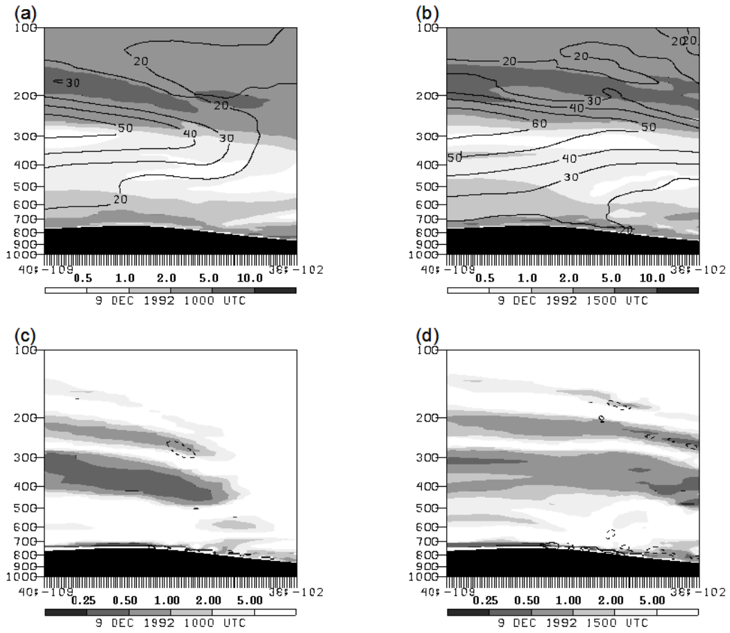
Figure A.2: Same as Fig. 2.11, except from 6 km smooth-terrain NHMSS simulation.
