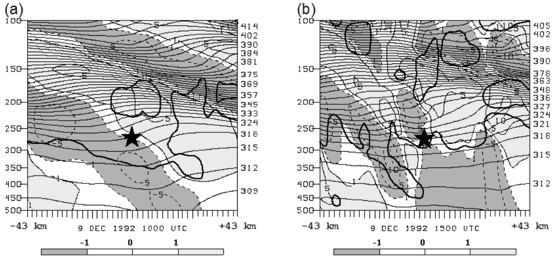
Figure 2.16: East-west vertical cross-section through aircraft incident location showing horizontal velocity divergence ( s^{-1} \times 10^{-4} , shaded), potential temperature (K, thin contours), and dynamic tropopause (2 PVU, bold contour) at (a) 1000 UTC and (b) 1500 UTC 9 December 1992. Aircraft incident denoted by star. Horizontal axis units equal to one grid length, vertical axis in hPa. From 2 km NHMASS simulation.
