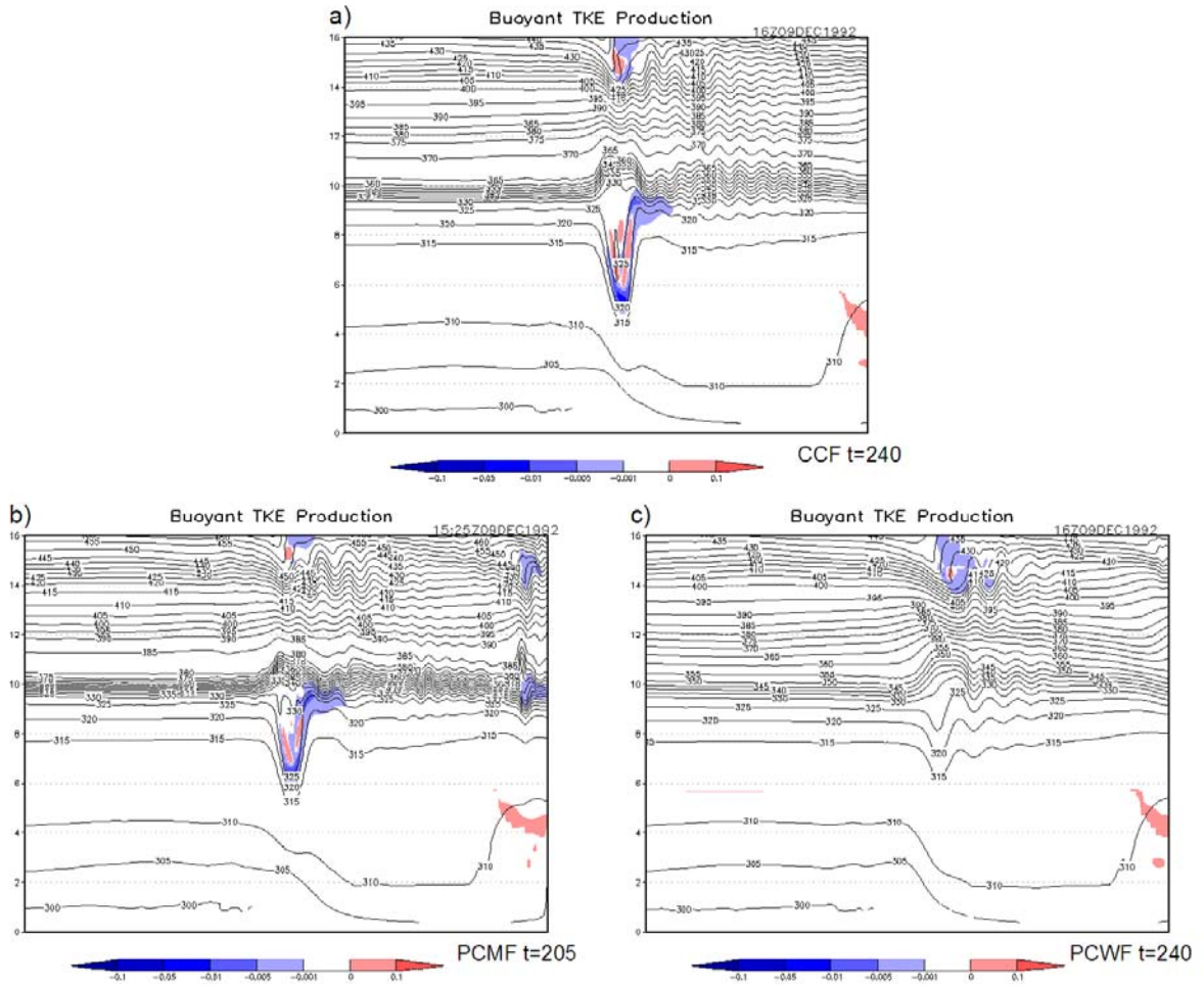
Figure 4.15: Buoyant production of TKE (shaded, m^2s^{-3} ) from Eq. (4.3) for (a) CCF (240 min), (b) PCMF (205 min), and (c) PCWF (240 min) simulations.
