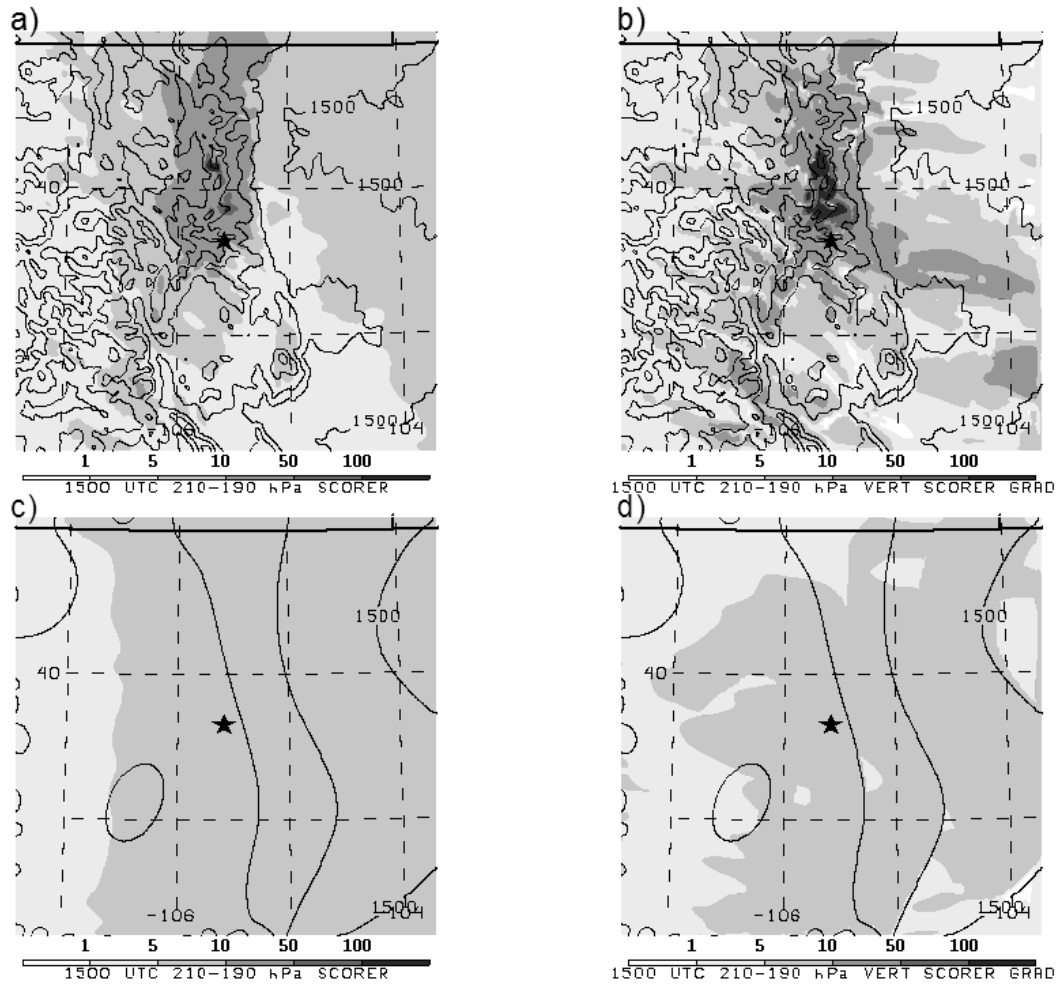
Figure A.6: 210-190 hPa layer (a,c) l^2 (shaded, m^{-2} \times 10^{-7} ) and \partial(l^2)/\partial z ( m^{-3} \times 10^{-10} ) valid 1500 UTC 9 December 1992 for the full-terrain (a,b) and smooth terrain (c,d) 2km NHMASS simulations. Terrain contours every 500 m. Aircraft incident location marked by star.
