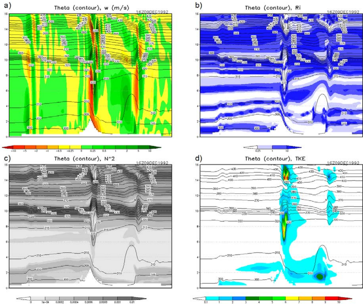
Figure 4.4: 2 km Colorado control simulation (CC) output at t = 240 min. Fields shown are (a) vertical velocity (shaded, \text{ms}^{-1} ), (b) gradient Richardson number (white means Ri < Ri_c ), (c) Brunt-Väisälä frequency squared (shaded, \text{s}^{-2} , darker shading indicates increased static stability), and (d) model-parameterized TKE (shaded, \text{m}^2\text{s}^{-2} ). In all panels, solid contours are of potential temperature (K), with 5 K interval for (a)-(c), and 10 K contour for (d) for clarity.
