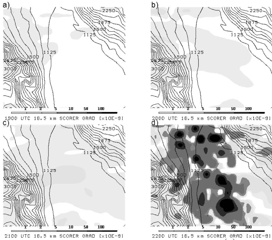
Figure 3.18: Simulated vertical gradient of the Scorer parameter (\partial(l^2)/\partial z) , \text{m}^{-3} \times 10^{-9} , shaded) for a portion of the 222 m WRF domain at 16.5 km MSL at (a) 1900 UTC, (b) 2000 UTC, (c) 2100 UTC, and (d) 2200 UTC 25 March 2006.
