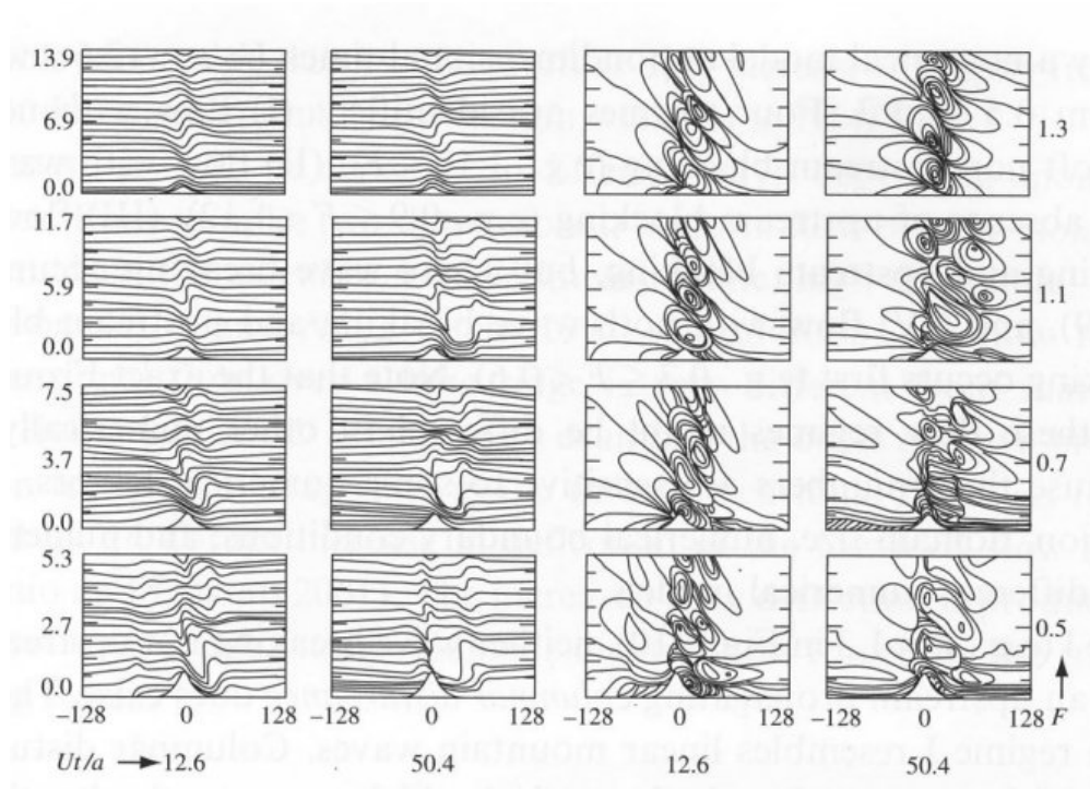
Figure 1.1: Two-dimensional numerical simulations of nonlinear responses to uniform, hydrostatic flow over a 1 km-tall bell-shaped mountain. Contours are potential temperature (left two columns) and perturbation u -wind (right two columns) for non-dimensional times Ut/a=12.6 and 50.4 , where U is the base-state mean wind and a is the mountain half-width (in this case 10 km). N=0.01 \text{ s}^{-1} in all cases, with U values of 5, 7, 11, and 13 \text{ms}^{-1} corresponding to F=0.5, 0.7, 1.1, \text{ and } 1.3 . From Lin (2007).
