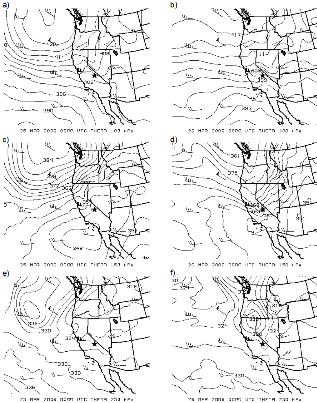
Figure 3.3: Potential temperature (K) and wind barbs ( \text{ms}^{-1} ) at (a-b) 100 hPa , (c-d) 150 hPa, and at (e-f) 250 hPa valid 0000 UTC 25 March 2006 (left column) and 0000 UTC 26 March 2006 (right column). Data from NCEP/NCAR North American Regional Reanalysis. The star marks the T-REX field site.
