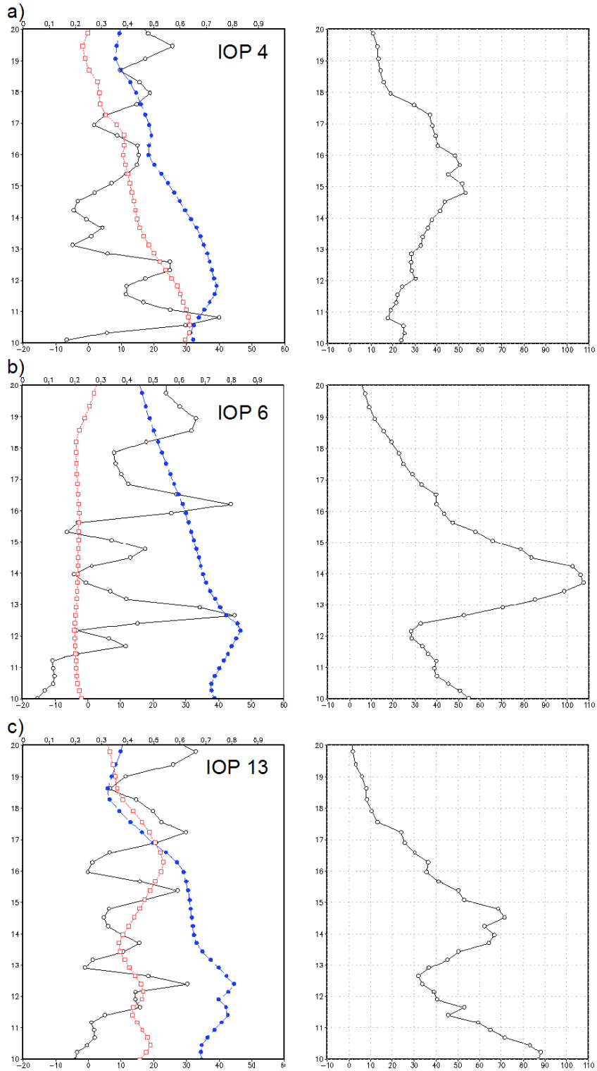
Figure 4.25: Vertical profile of initialization N^2 (black, x values on upper axis, \text{s}^{-2} \times 10^{-4} ), u (blue, lower x axis, \text{ms}^{-1} ), and v (red, \text{ms}^{-1} ) on left, and all-time maximum TKE ( \text{m}^2\text{s}^{-2} ) in the 10-20 km layer for the right half of the domain for IOPs (a) 4, (b) 6, and (c) 13 (cases with strong stratospheric wave action).
