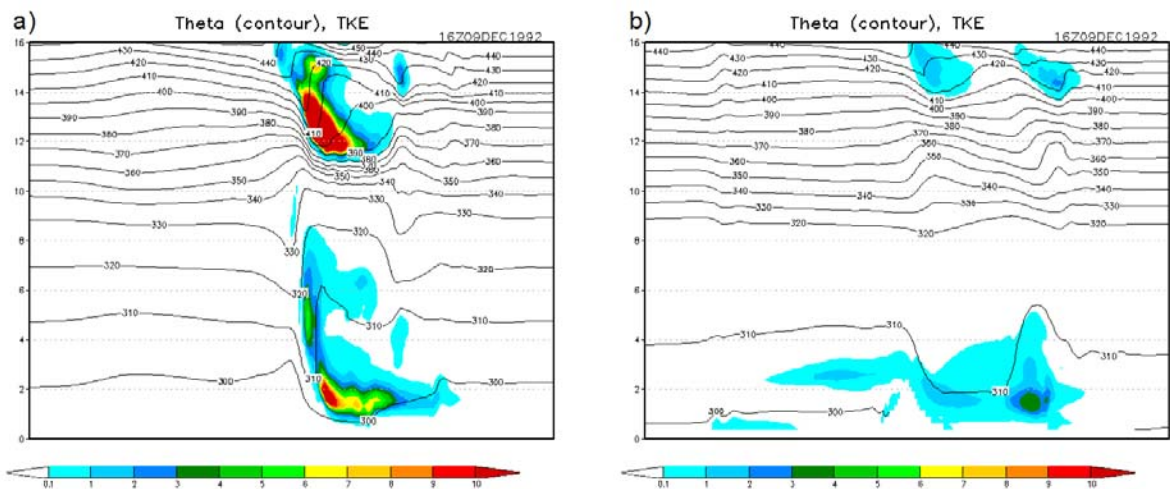
Figure 4.7: Model parameterized TKE (shaded, \text{m}^2\text{s}^{-2} ) and potential temperature (contoured, K) at t = 240 min for (a) PCS and (b) PCI simulations.
