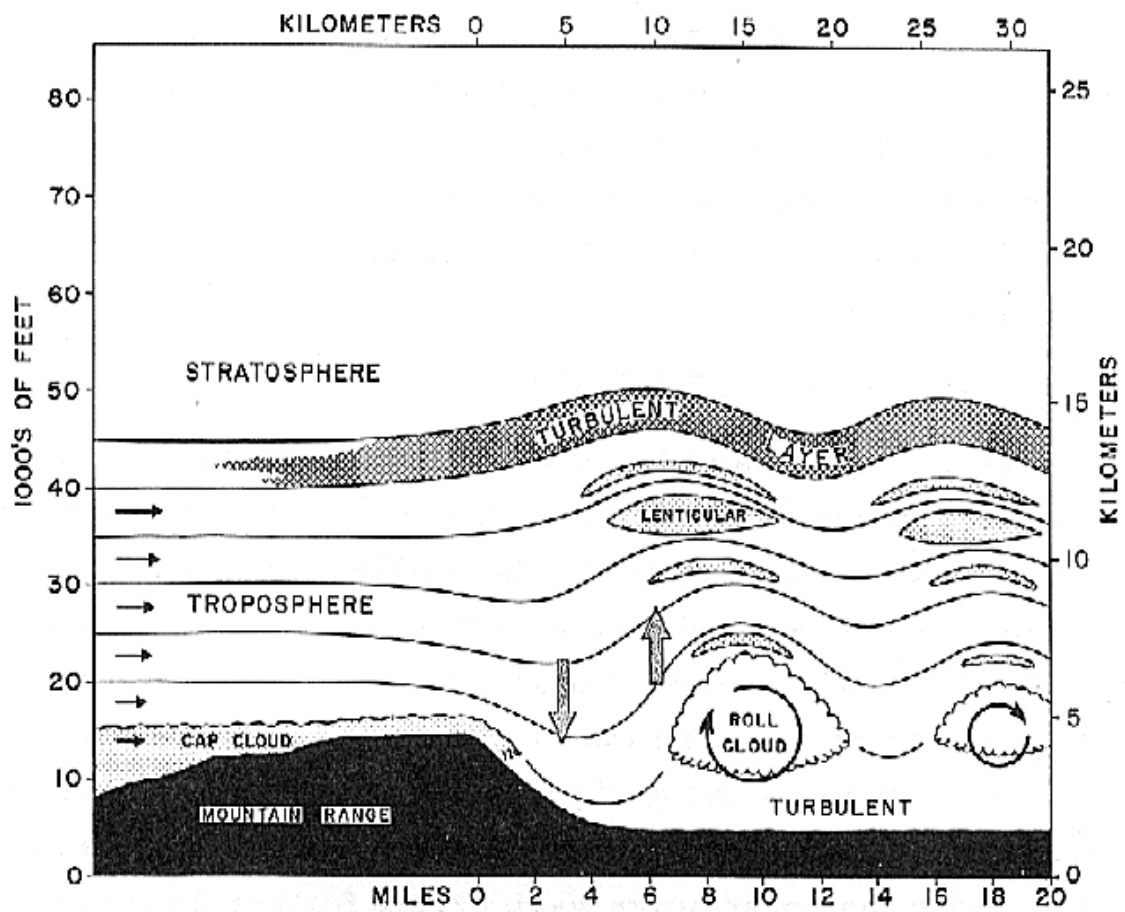
Figure 1.4: Schematic of flow over a mountain with a rotor and roll cloud (from Kuettnner 1959).
