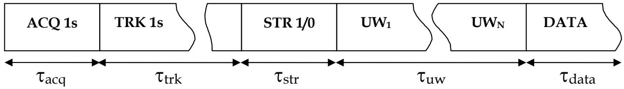
Figure 8- DSSS Signalling Packet Structure
