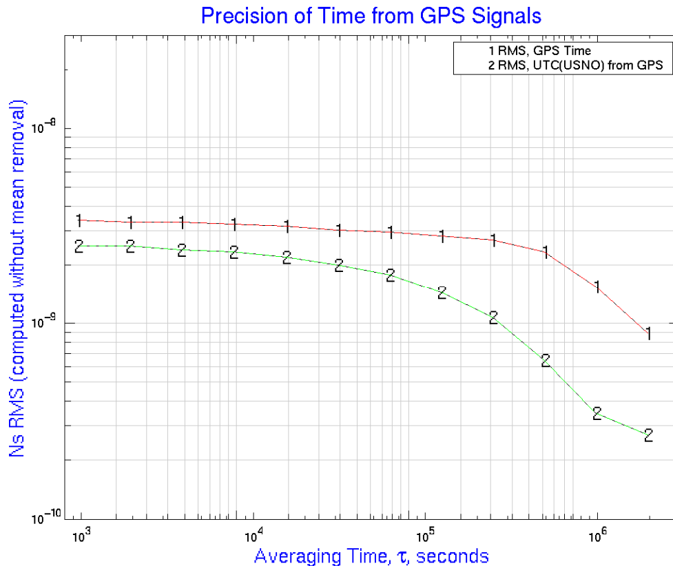
Figure 4. The precision of GPS Time and of GPS's delivered prediction of UTC (USNO), using TTR-12 data from 11JUL02 to 16DEC04, measured by the attainable external precision (rms, mean not removed) as a function of averaging time, and referenced to UTC (USNO). Improved performance in the predictions of UTC (USNO) could be realized if only the most recently updated navigation messages are used. The attainable accuracy is the precision degraded by the error of the user's calibration relative to the USNO GPS receivers.
