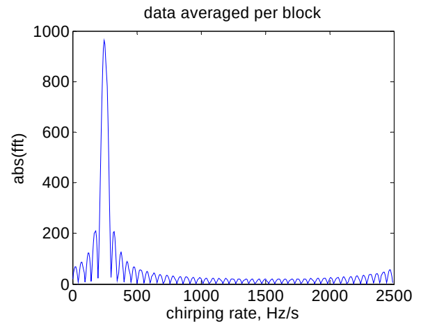
Fig. 4. FFT Applied to Samples Averaged per Block
