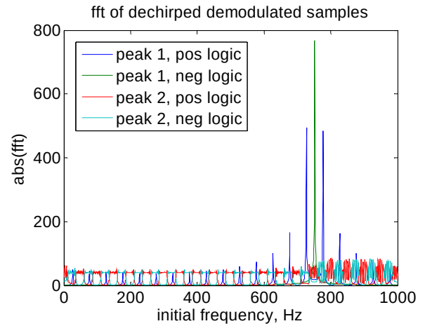
Fig. 6. FFT of Dechirped and Demodulated Samples
