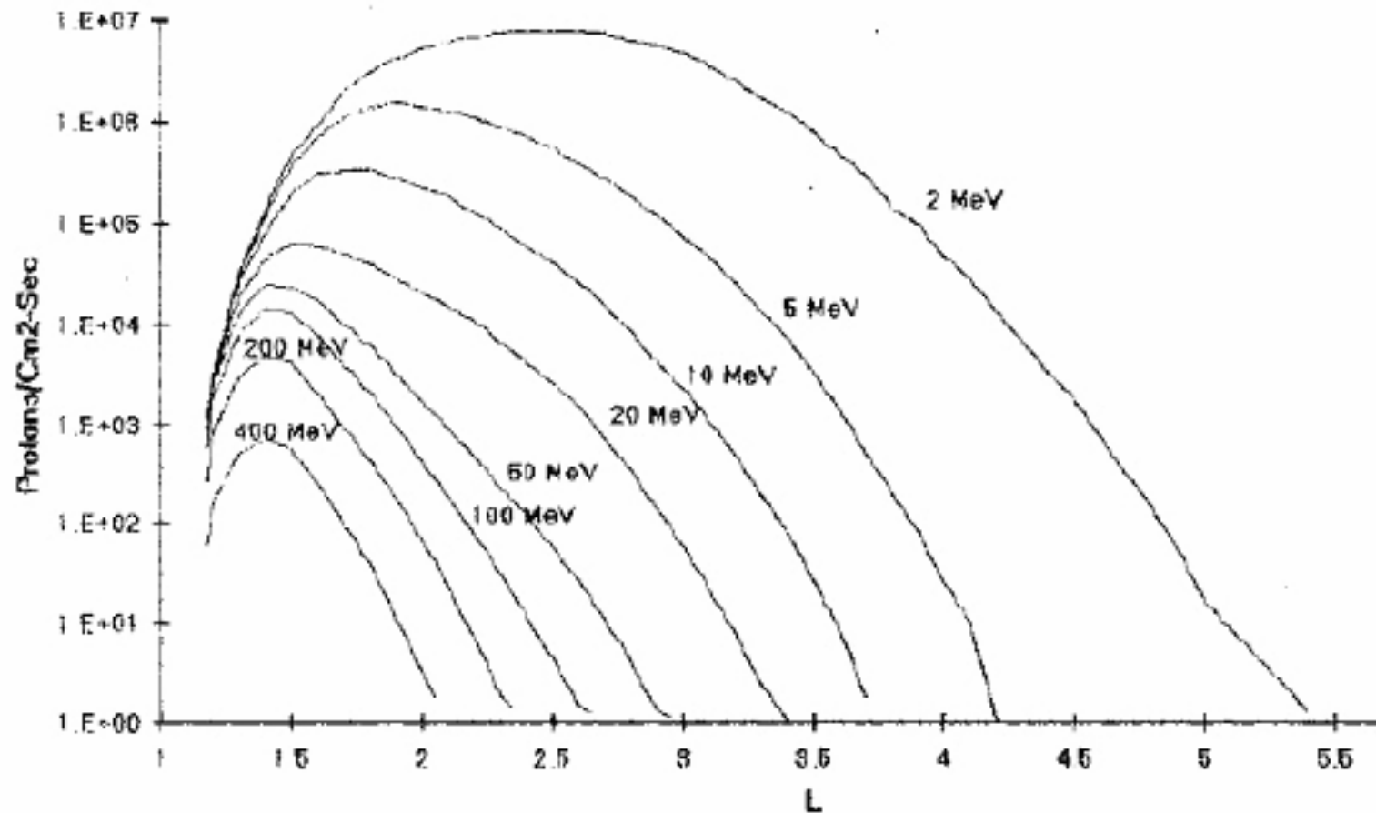
Figure 2.3: High energy proton fluxes and energies as a function of L-value from the AP8MIN model [3].
