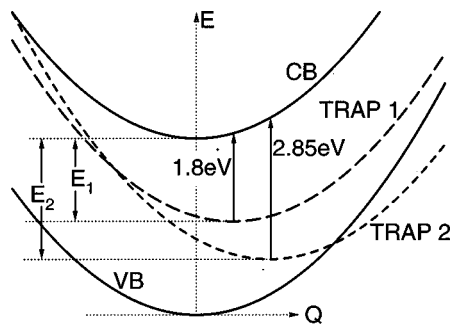
FIG. 3. Sketch of a configuration coordinate diagram showing the relationship of the deep traps and the band edge. E_1 and E_2 represent the thermal trap depths, while the optical transition energies indicate the photoionization thresholds determined in the present work.
