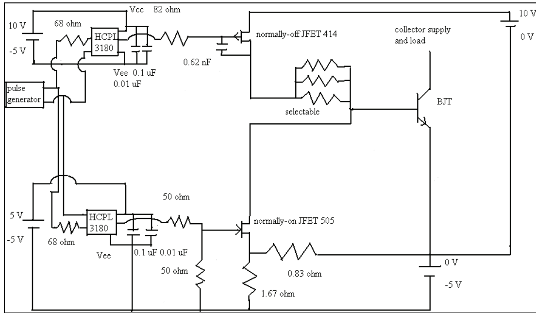
Figure 1. JFET Drive Circuit for BJT base.
