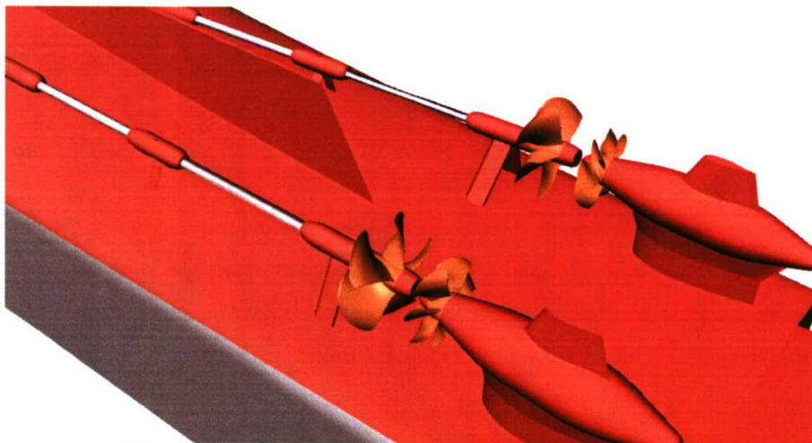
Figure 6. An isometric view of the Shaft-Pod configuration.
