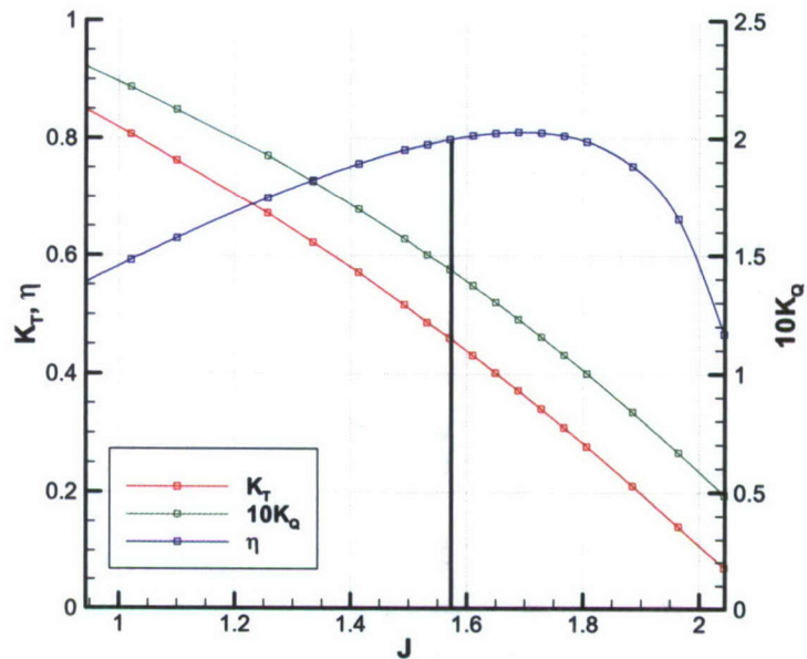
Figure 30. The combined open water curves.
