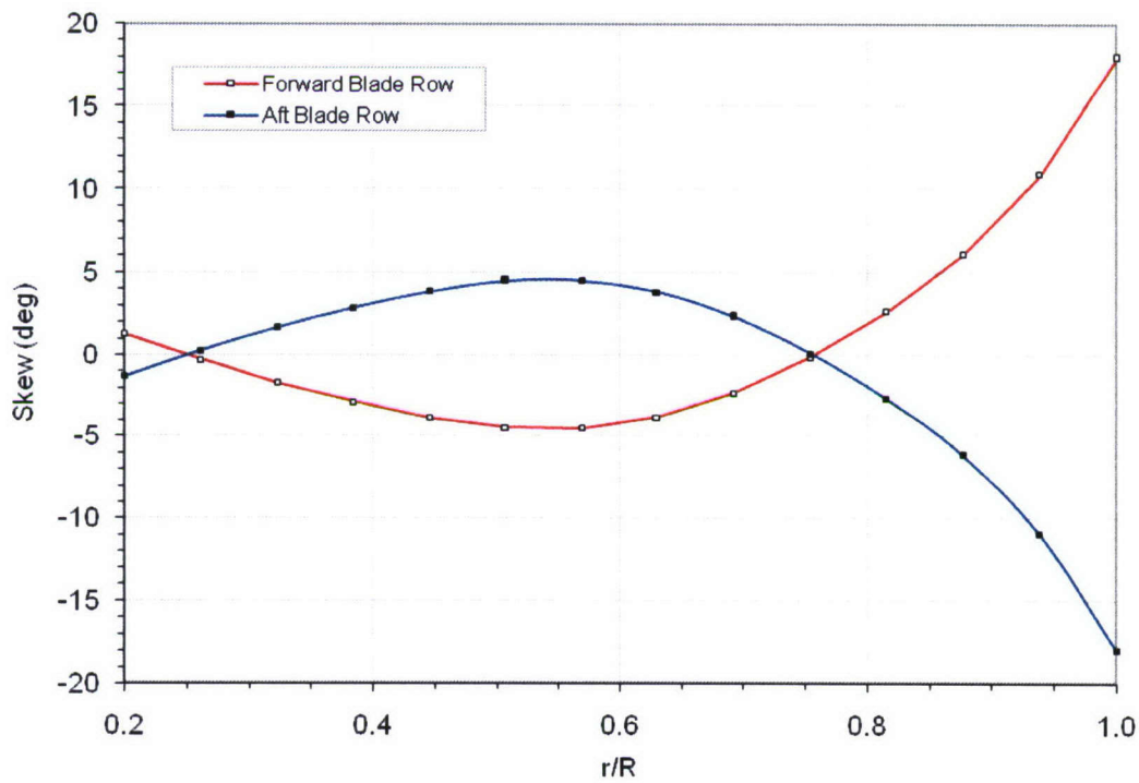
Figure 20. The skew distribution for the forward and aft blade rows.
