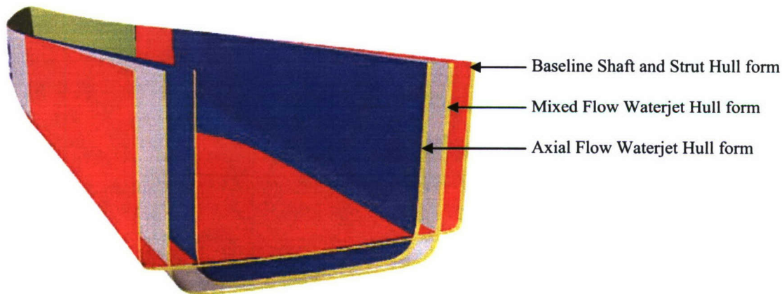
Figure 1. The three different JHSS hull forms.
