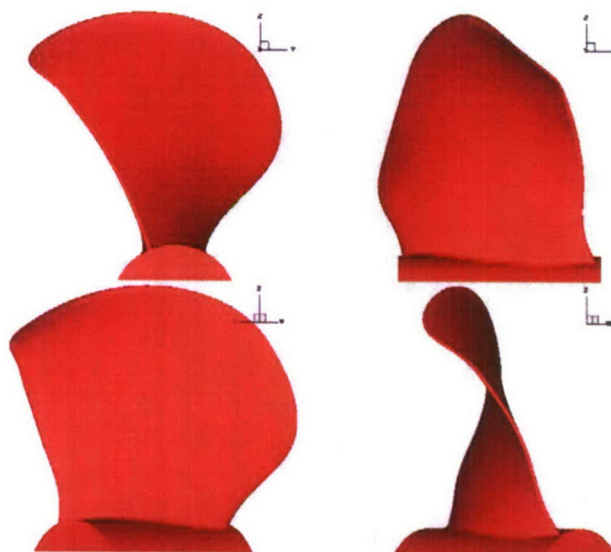
Figure 24. 3D views of one blade of the forward propeller.
