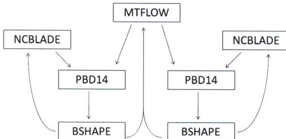
Figure 22. A flowchart showing the relationships between the codes used during the detail design.
