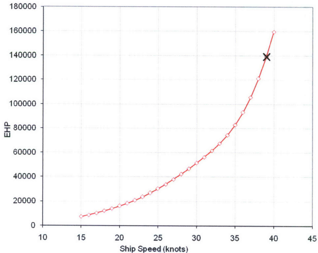
Figure 9. The effective horsepower (EHP) curve for the Shaft-Pod configuration.
