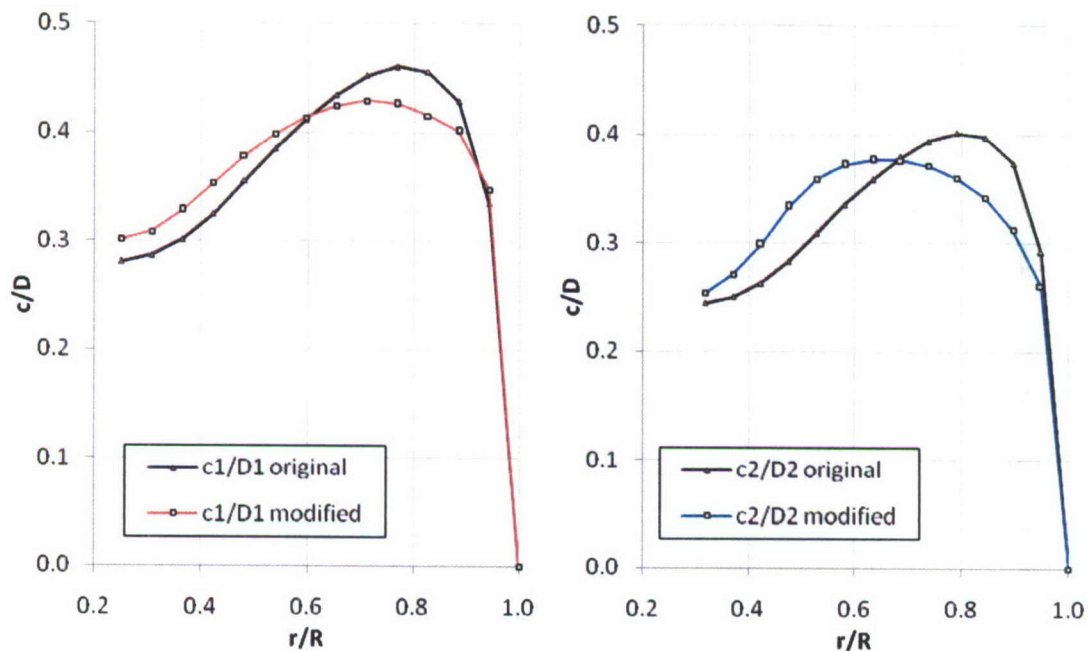
Figure 17. The initial and modified chord distributions.
