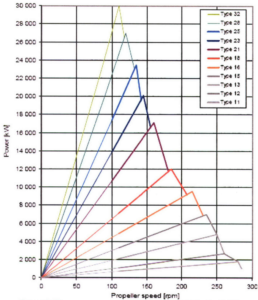
Figure 13. The power ranges and RPMs of different Azipod units [3].
