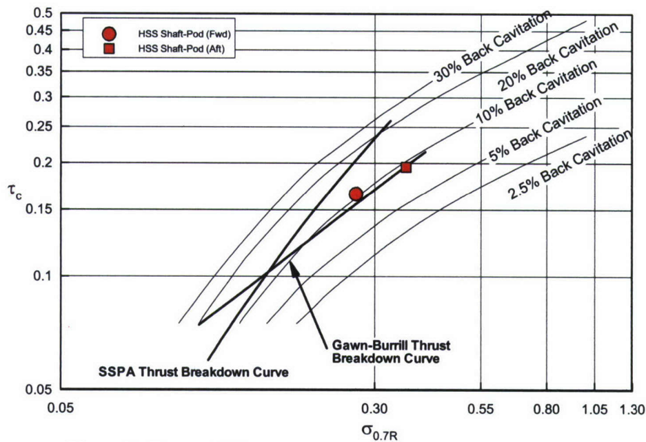
Figure 21. The two HSS propeller designs shown on the Burrill chart.
