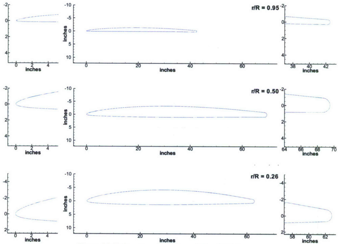
Figure 29. Full scale section views of the aft blade row.
