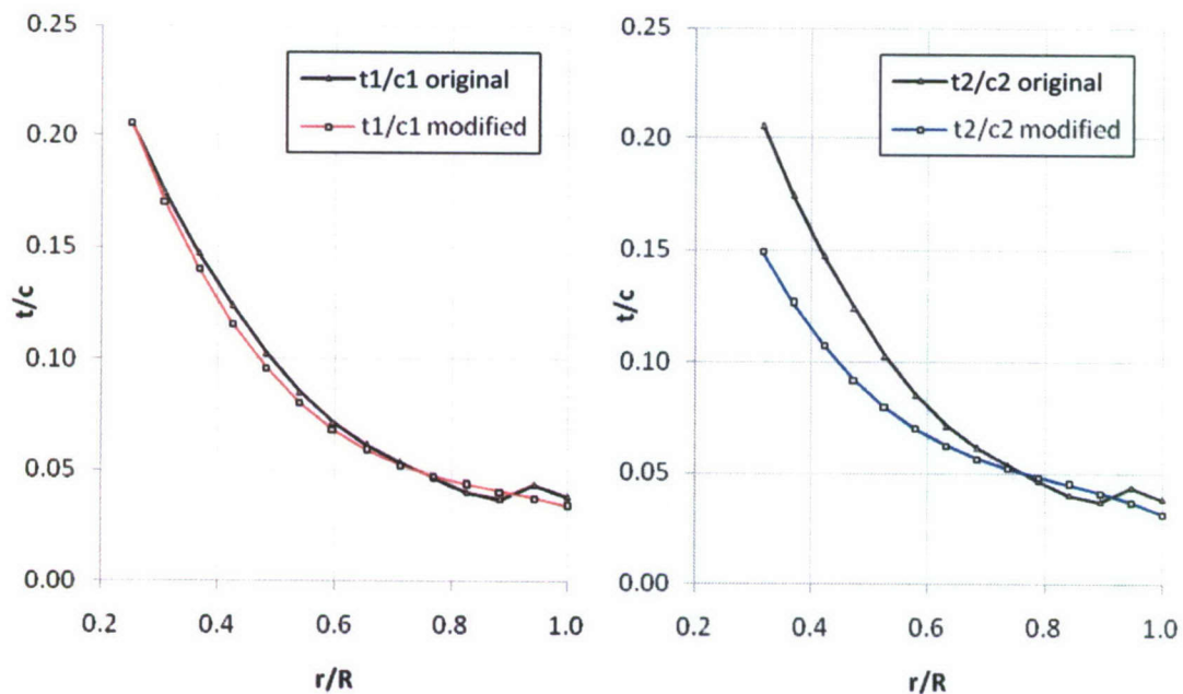
Figure 18. The initial and modified thickness distributions.
