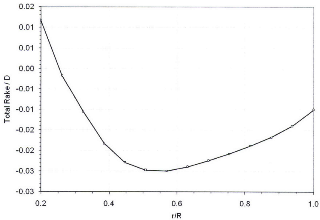
Figure 19. The rake distribution for both blade rows.
