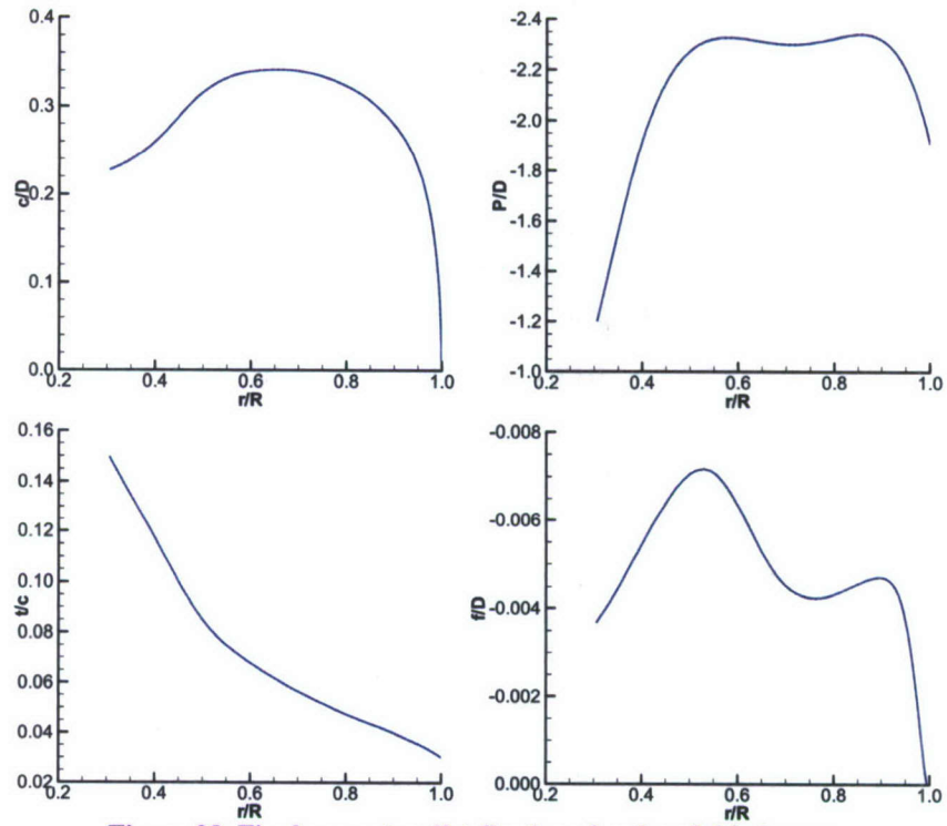
Figure 28. Final geometry distributions for the aft blade row.
