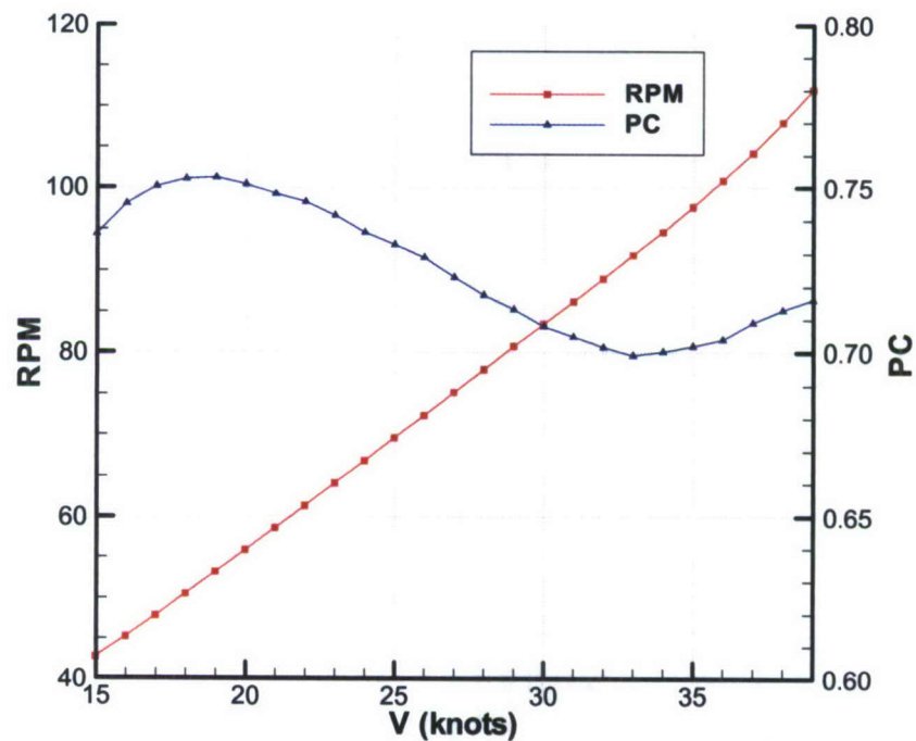
Figure 31. The combined powering curve.
