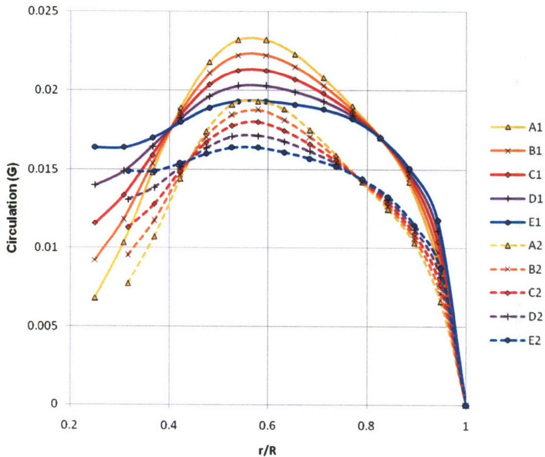
Figure 15. The initial and optimal circulation distributions and the circulation distribution compromises.
