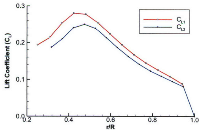
Figure 16. The lift coefficient distributions after changes to the chord, thickness, and circulation distributions.
