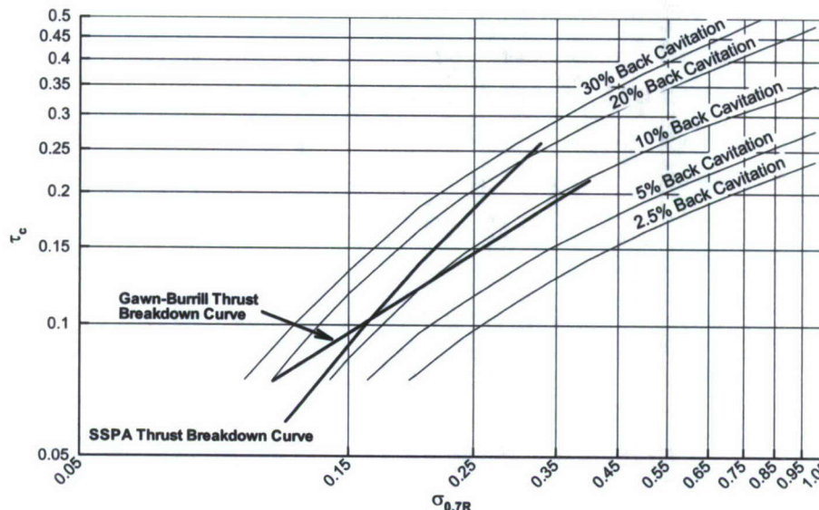
Figure 12. The Burrill chart.
