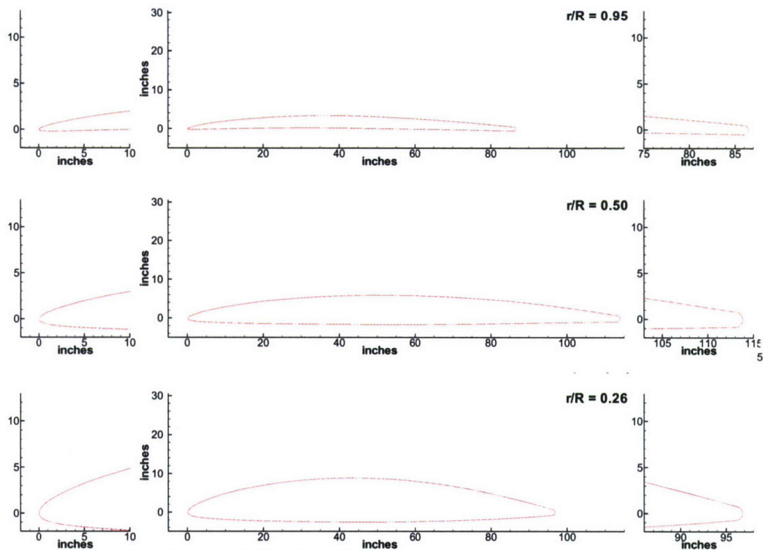
Figure 26. Full scale section views of the forward blade row.
