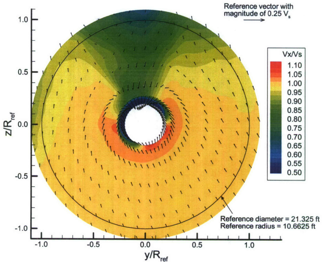
Figure 10. The JHSS BSS inboard starboard wake survey.
