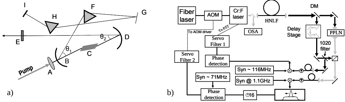
Fig. 1. a) Laser cavity configuration. b) Servo control schematic used to lock f_i and f_o .
