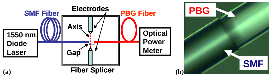
Fig. 1. (a) Experimental set-up for the measurement of splice losses. A tunable diode laser at 1550 nm is used with an optical power meter to measure the coupling during the splice procedure using a commercial arc splicer. (b) A micrograph showing the splice between the SMF and PBG fiber. Picture courtesy of the GaN Group at KSU Physics.
