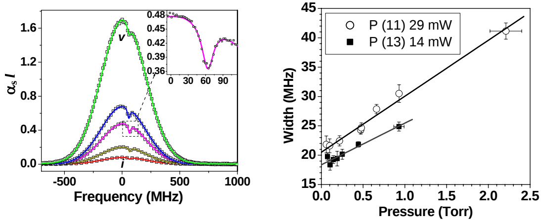
Fig. 2. (left) \alpha_s I calculated with pressure varying from v to i according to the legend of Fig. 1. Solid lines represent fits to the above equation, using the function described above. (right) Width vs. pressure resulting from fits at left.
