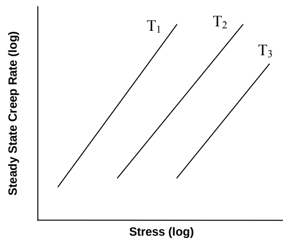
Figure A-3. Minimum Creep Rate vs Applied Stress
