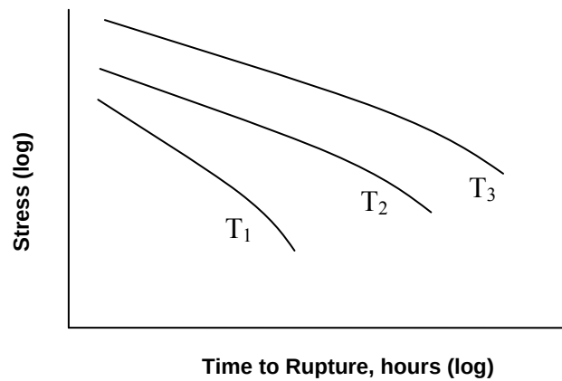
Figure A-2. Typical Stress Rupture Curve at Different Temperatures
