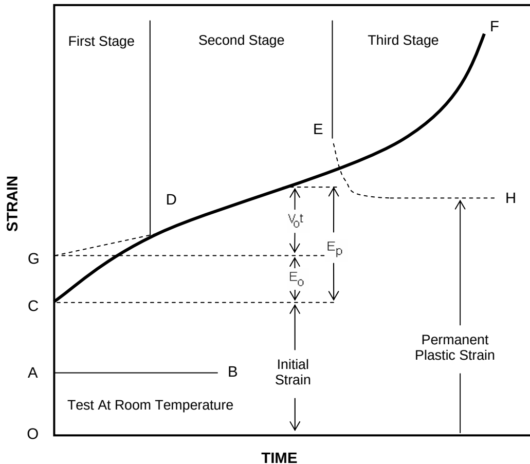
Figure A-1 Strain vs Time
