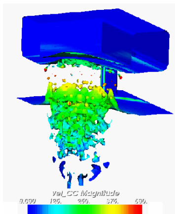
Fig. 6. Simulation of DRDC Case using full MPMICE.
