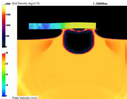
Fig. 5. Simulation with tightly coupled MPMICE-DYNA3D.
